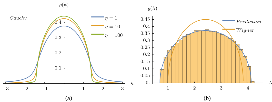
Figure 3: (a) Limiting distribution of the rescaled eigenvalues \kappa = \lambda/\sqrt{4\eta} , with \rho(\lambda) given in Eq. (49) for the Cauchy case (see Section 2.4.1). In this plot we used \mu = 0 and \omega = 0.5 . (b) Distribution of the eigenvalues \rho(\lambda) in the case in which p_a(a) is the Wigner semicircle distribution (see Section 2.4.2), and numerical check of the prediction in Eq. (56). The histogram was built using r = \sqrt{2} , \mu = 1 + \sqrt{2} , \nu = 1 , \gamma = 1.1 and N = 2000 .
