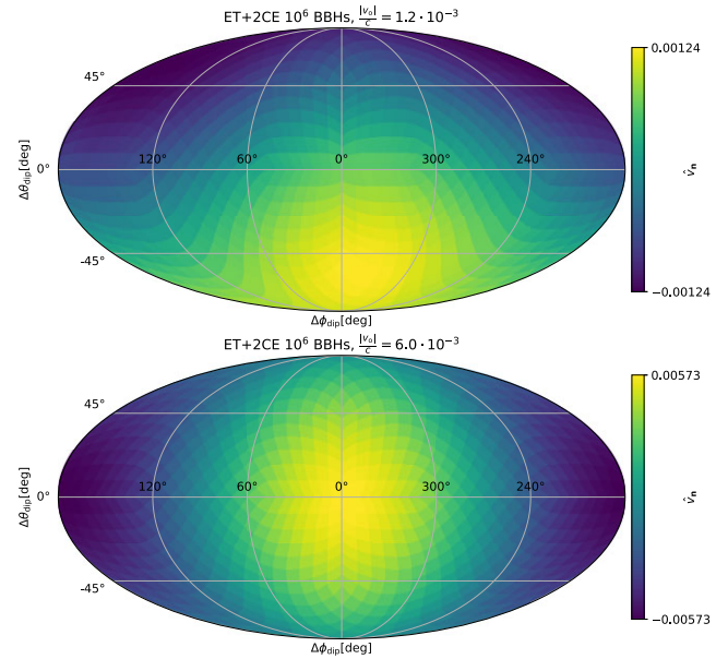
Figure 3. Sky distribution of the estimator \hat{v}_n for the CMB fiducial value (top map) and the AGN fiducial value (bottom map). The maps are centred around the injected direction of the observer velocity. The figure is generated by dividing the sky in equal size pixels of 53 \text{ deg}^2 .
