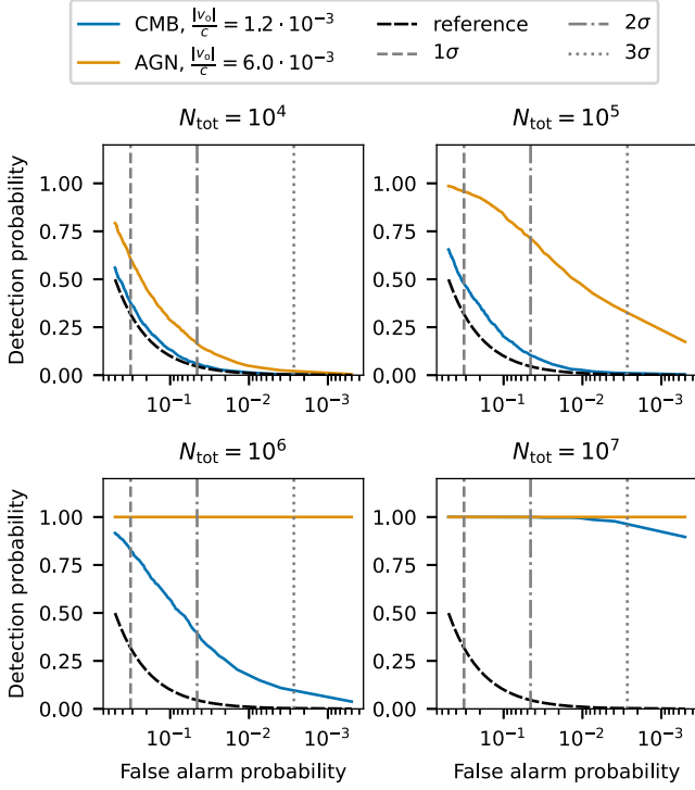
Figure 6. FAP versus detection probability plots for the injected CMB and AGN fiducial values (blue and orange lines). The vertical-dashed lines indicate the FAP at the standard 1\sigma , 2\sigma , 3\sigma credible intervals. The black-dashed line is the reference to indicate when the detection probability coincides with the FAP (they are the same distribution).
