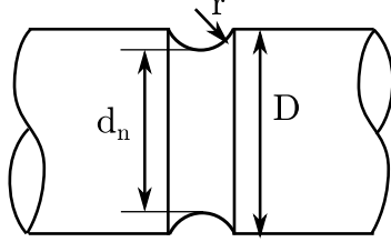
Fig. 27. Notch shape: D = 7 mm, d_n = 5.6 mm, r = 1.2 mm.
