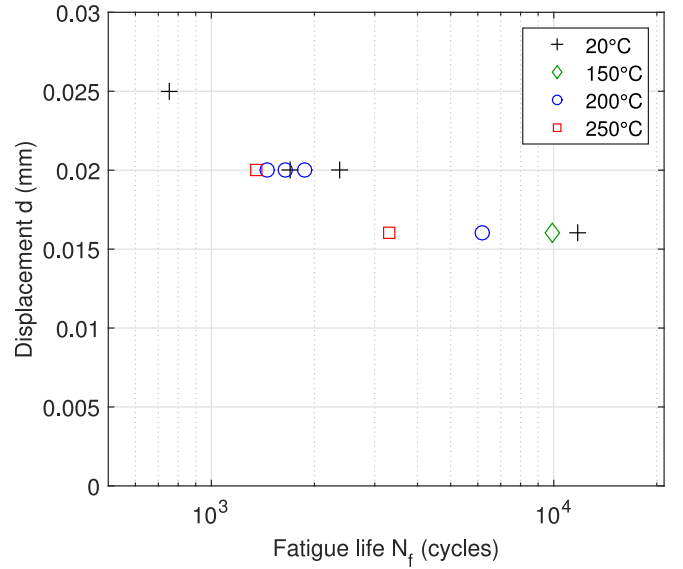
Fig. 28. Fatigue life for notched specimens ( K_t = 1.78 ).
