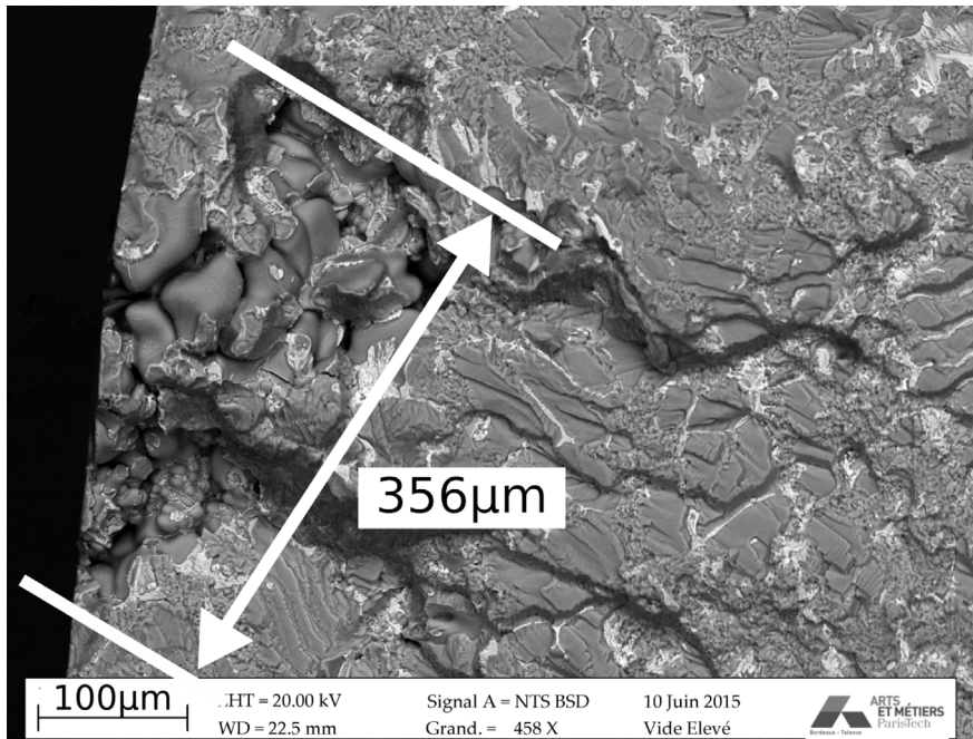
Fig. 2. Measurement of defect size (Specimen 87T5, \Delta\epsilon/2 = 0.30\% , 20^\circ\text{C} , R_f = -1 , N_f = 2904 cycles).
