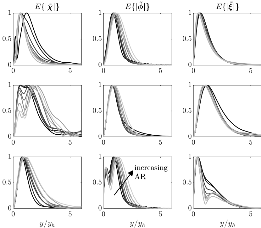
FIGURE 13. Mean self-similar modes for \chi (left), \phi (center) and \xi (right). Rows correspond to the x -, y - and z -components from top to bottom.
