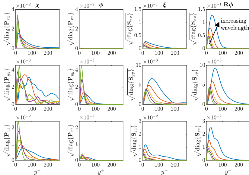
FIGURE 6. Comparison of the wall-shear-associated forcing modes obtained by RESPOD (1st column) and RBE (2nd column), respectively, and the corresponding velocity fields (3rd and 4th columns, respectively) respectively, at \lambda_x^+ = 341, 487, 682, 1137 and 1706 with \lambda_x^+/\lambda_z^+ = 6 .
