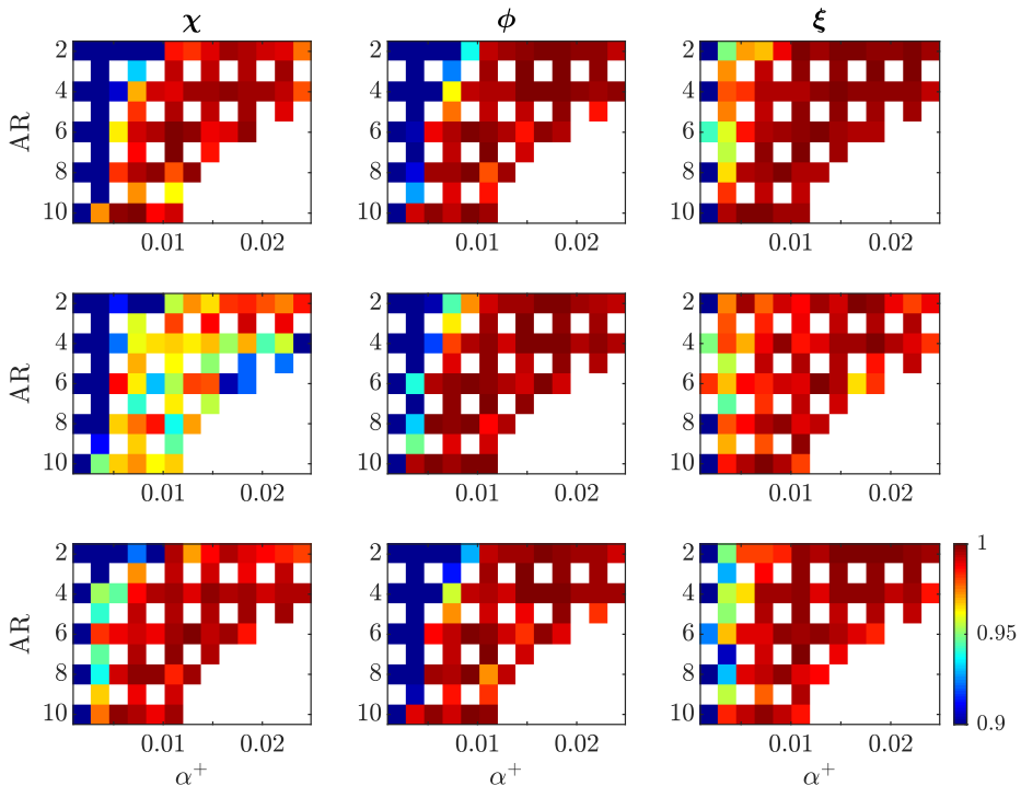
FIGURE 12. Self-similarity maps, \gamma_\chi (left), \gamma_\phi (center), and \gamma_\xi (right) for different ARs and \alpha^+ values. Rows correspond to the x -, y - and z -components from top to bottom.
