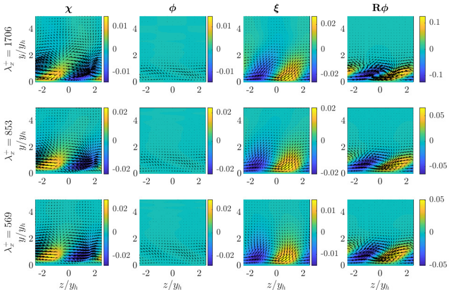
FIGURE 9. Reconstruction of wall-shear-associated forcing modes, \chi (1st column) and \phi (2nd column) and the corresponding velocity fields (3rd and 4th columns, respectively) in the y - z plane at three wavenumbers (from top to bottom). Color-plots indicate the x -component while vectors show y - and z -components. The domain is rescaled using y_h for each wavenumber.
