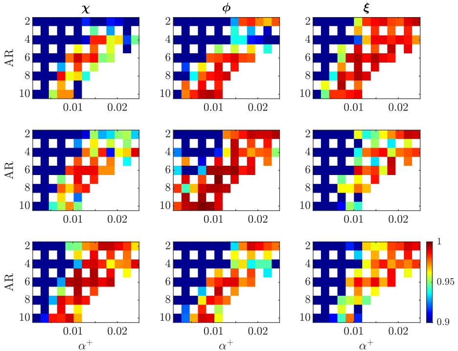
FIGURE 18. Self-similarity maps, \gamma_\chi (left), \gamma_\phi (center), and \gamma_\xi (right) for different ARs and \alpha^+ values obtained at sub-dominant frequencies. Rows correspond to the x -, y - and z -components from top to bottom.
