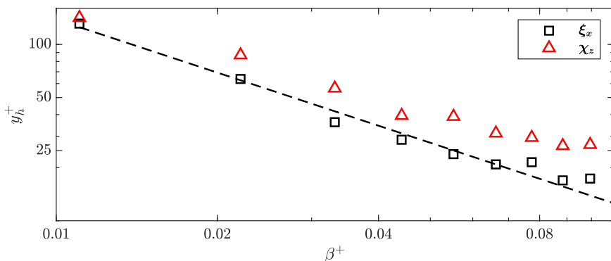
FIGURE 8. Mode center, y_h^+ obtained using \xi_x (square) and \chi_z (triangle) at different wavenumbers with AR=6. The dashed line shows 1/\beta^+ trend.
