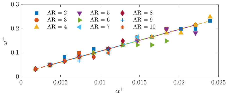
FIGURE 10. Peak-energy containing frequencies for different wave number pairs with fixed AR. Different markers indicate different AR values. The coloured dashed lines correspond to the best-fit lines for different ARs using the same color code.
