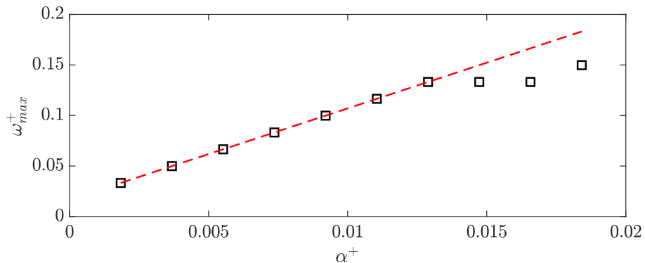
FIGURE 3. Maximum-energy-containing frequency, \omega_{max} of spanwise wall shear, \tau_z for different Fourier-mode pairs with AR=6. The red-dashed line indicates the best-fit minimizing L_1 -norm error.
