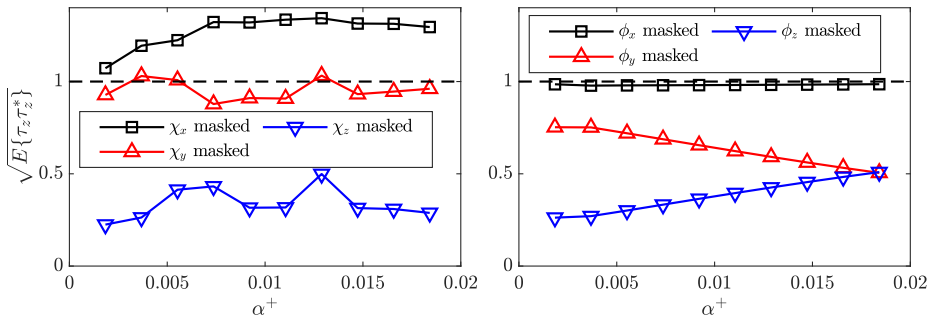
FIGURE 7. Square root of PSD of \tau_z obtained using partially masked \chi (left) and \phi (right) at different wavenumbers with AR=6. Unmasked PSDs are all unity, shown by the dashed line.
