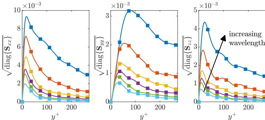
FIGURE 4. PSD of the response, \hat{\mathbf{q}} , (solid lines) in comparison to its resolvent-based prediction, \mathbf{R}\hat{\mathbf{f}} , (markers) at \omega_{max} for different Fourier-mode pairs with AR=6. Wavelengths plotted are \lambda_x^+ = 487, 569, 683, 853, 1137, \text{ and } 1706 .
