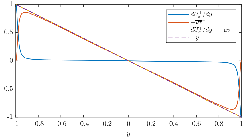
FIGURE 1. Momentum budget plot for the DNS of the channel flow.
