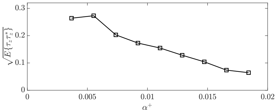
FIGURE 5. Amplitude spectral density of spanwise wall shear, \tau_z at \omega_{max} for different Fourier-mode pairs with AR=6.
