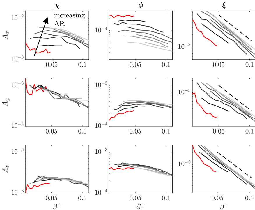
FIGURE 14. Mode amplitudes for \chi (left), \phi (center) and \xi (right) at different wavenumber pairs. Rows correspond to the x -, y - and z -components from top to bottom. ARs range from 2 to 10. AR=2 is shown with red and the rest with gray scale. Dashed lines indicate 1/(\beta^+)^2 trend.
