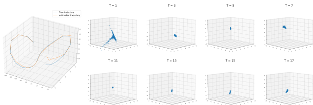
Figure 7: Left : true and inferred Lorenz-63 states and states, right : sampling of 1000 points of the inferred posterior p(x_T|y_{1:T}) for different value of T. It clearly illustrates the ability of the proposed framework to address non-Gaussian features.
