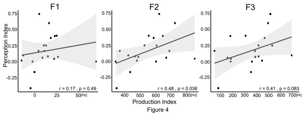
Figure 4. Scatterplots of perception index (PSE differences) against production index (differences between /e/ and /ø/ in F1, F2 and F3). Solid lines represent the regression line and the shaded area represents 95% confidence intervals.
