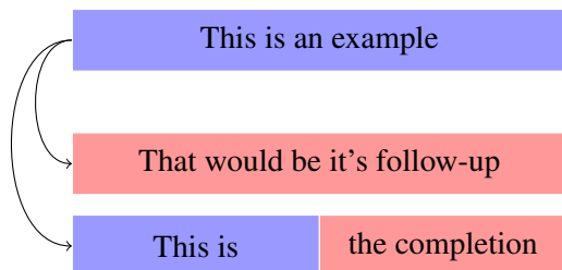
Figure 2: Generation methods examples. In blue is the initial example and in red is the generated text. The first generated example is from sentence follow-up, and the second is from sentence completion.
