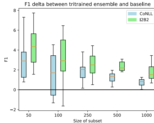
Figure 4: Boxplot of CoNLL and I2B2 deltas between tri-trained ensemble and baseline ( \Delta ensemble). For each subset size, the left boxplot is CoNLL, the right boxplot is I2B2.
