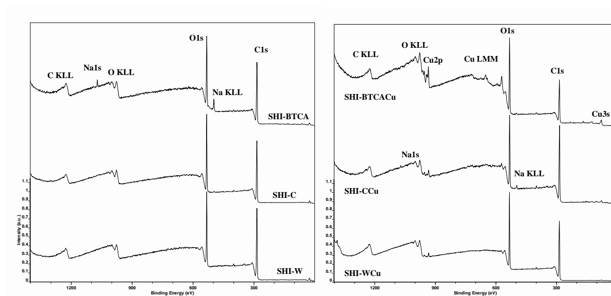
Fig. 7. XPS wide scan spectra of shives before (left) and after (right) copper adsorption.
