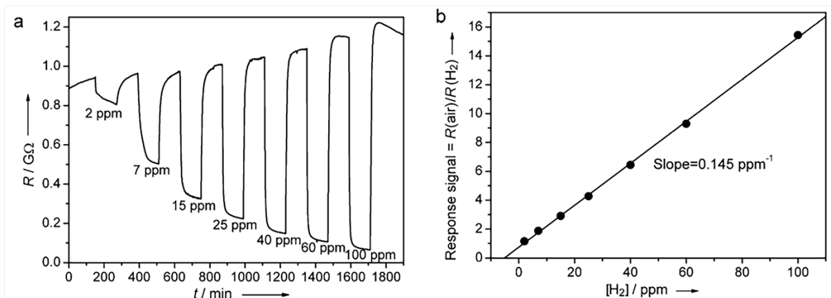
Figure 17. (a) Resistance change and (b) response signal of a W_{18}O_{49} nanowire thin film with respect to various concentrations of H_2 at room temperature. Source: adapted from W. Cheng et al. [126] with permission of Wiley-VCH Verlag GmbH & Co. KGaA.
