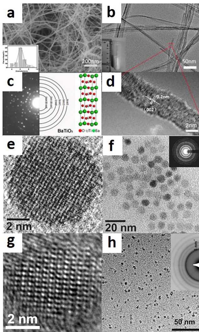
Figure 5. Electron microscopy images and selected area electron diffraction (SAED) of \text{BaTiO}_3 (a-d) ultrathin nanowires, nanoparticles obtained in (e-f) diphenylether and oleic acid and (g-h) benzyl alcohol synthesis. Source: adapted from (a-d) Yang et al. [48], Copyright 2013, (e-f) from O'Brien et al. [50], Copyright 2001 and (g-h) from Niederberger et al. [54], Copyright 2004, with permission of American Chemical Society.
