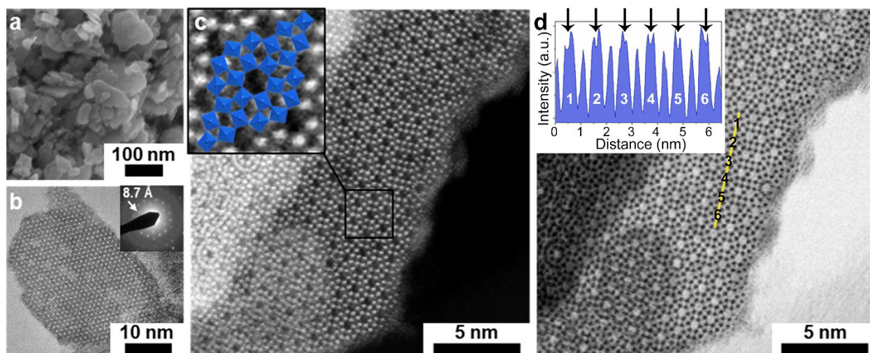
Figure 20. (a) SEM and (b) TEM images of \text{H}_{0.07}\text{WO}_3 hexagonal bronze nanoplatelets. inset in (b) shows a typical SAED pattern. (c) HAADF-STEM and (d) ABF-STEM micrographs showing the arrangement of tungsten octahedra (blue, inset of c). Source: adapted from J. Besnadiere et al. [138] with permission of Springer Nature.
