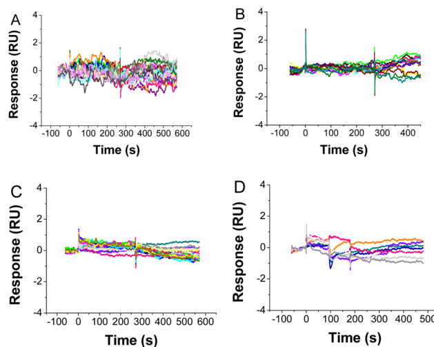
Fig. 3 Sensorgrams recorded during the interaction of L-Tym (concentrations ranging from 10 nM to 25 μM) on the active flow cell after the double-reference-subtraction procedure for: (A) Apt 23 -T 3 -Biot, (B) Apt 23 -T 6 -Biot, (C) Apt 23 -T 9 -Biot and (D) Apt 23 -T 12 -Biot. T = 25 °C. Flow rate: 30 μL min -1 . Sensorgrams for Apt 23 -A 6 -Biot are presented in Fig. SI-12†.
