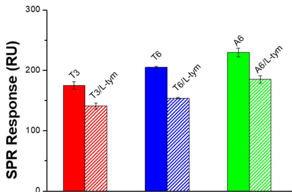
Fig. 5 SPR response recorded for the injection of Apt 23 bearing various spacers on a gold surface protected by a pegylated self-assembled monolayer. (Plain) 100 μM of aptamer; (hatched) 100 μM of aptamer with 1 mM of L-Tym in running buffer. T = 25\text{ }^{\circ}\text{C} . Apt 23 -T 3 (Red), Apt 23 -T 6 (Blue), 13 Apt 23 -A 6 (green).
