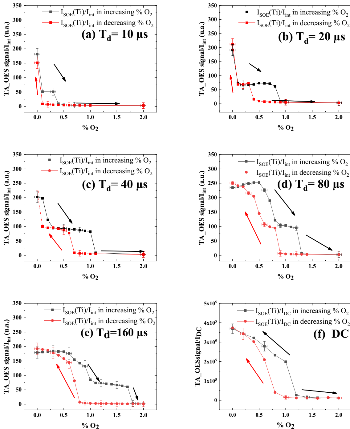
Fig. 8. Hysteresis for different pulse widths in function of O 2 percentages. (a) 10 μs, <P> T = 46 W; (b) 20 μs, <P> T = 49 W (c) 40 μs; <P> T = 51 W (d) 80 μs, <P> T = 49 W; (e) 160 μs, <P> T = 47 W and (f) DC, P = 45 W. The pressure is 1.4 Pa and the HiPIMS period is 1 ms.
