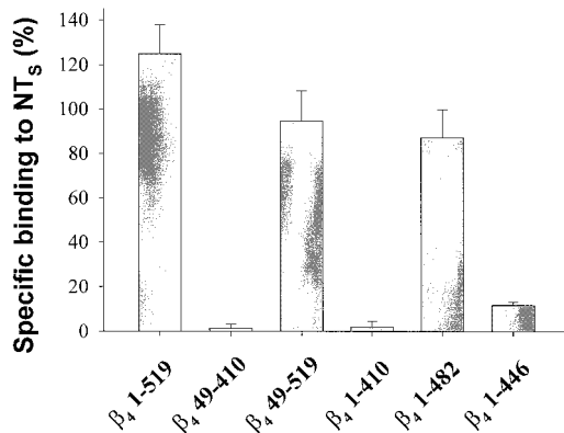
FIG. 6. The carboxyl terminus of \beta_4 is also involved in NT S binding. ^{35} S- \beta_4 and deleted derivatives were assayed for their capacity to interact with GST-NT S (5 \mu M). Specific binding was calculated by subtraction of binding to GST (at the same concentration) and normalized by expression as a percentage of maximal binding to GST-AID A (500 nM). Error bars represent normalized S.D.
