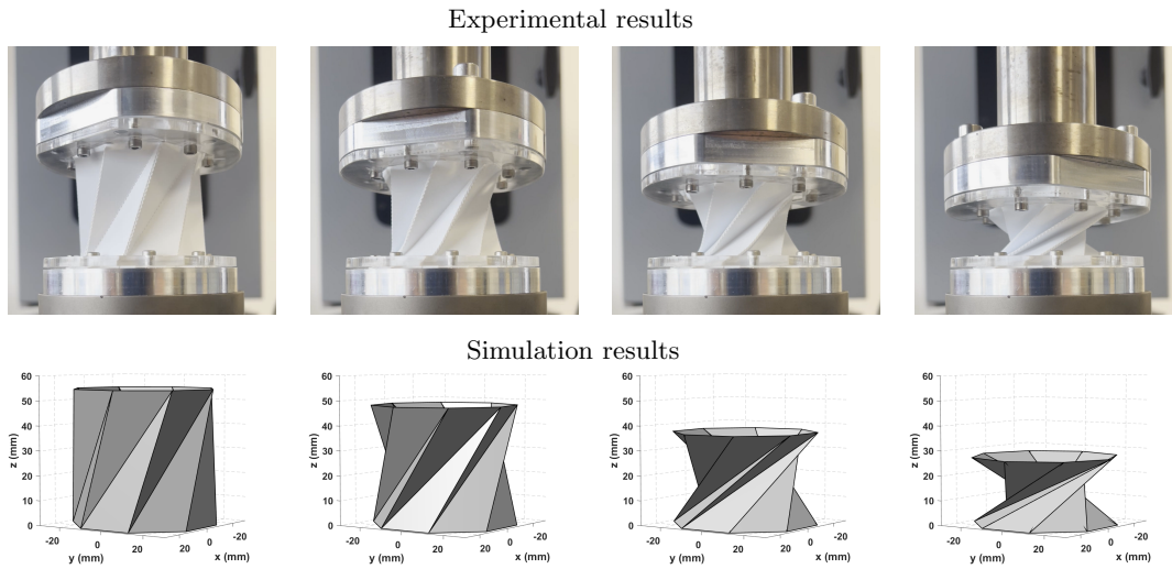
Figure 9: An example of the folding process comparison according to Origami Kresling tower: The photos on top show the incremental state during folding. The images show the simulation results according to corresponding displacements. The model can provide an accurate description of the folding kinematic of structure.
