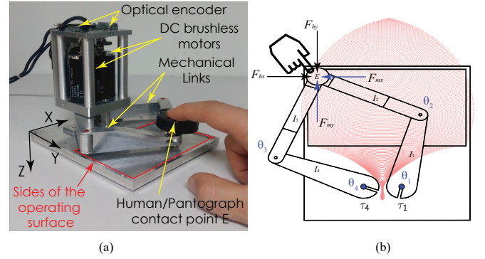
Fig. 1. (a) Pantograph: a bilateral haptic interface. (b) Schematic representation of the pantograph.
