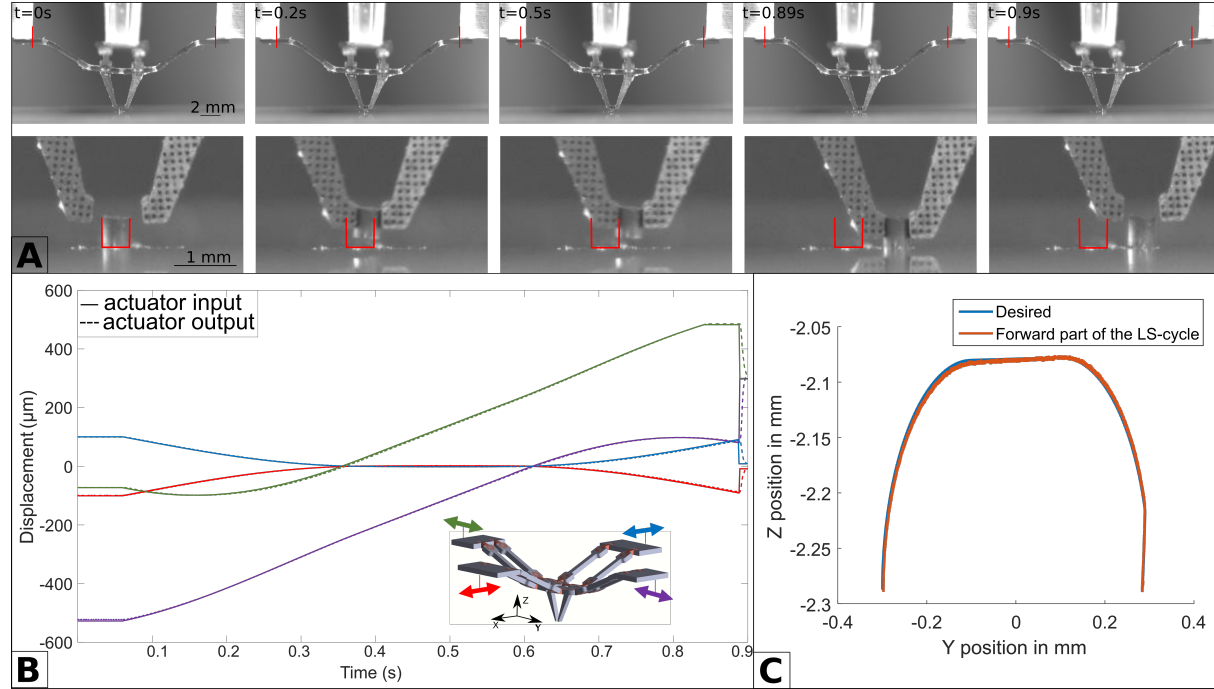
Fig. S3. Analysis of the forward part of the LS-cycle (Low Speed - 2 s) pick-and-place cycle. The manipulated object is a 350 \mu m diameter and 400 \mu m height silicon cylinder and the result is presented for the forward part of the LS-cycle which can be considered as quasi-static. A- Motion capture of the first 0.9 s of the LS-cycle where the manipulator grasps and moves the object from the initial position to the final one. Initial positions of the actuators and the object are represented in red; B- Command vector of each actuator versus the output vector during the first 0.9 s of the LS-cycle; C- Trajectory of the end-effectors in the (OYZ) plan for the reference cycle (blue), during the first 0.9 s of the LS-cycle (red).
