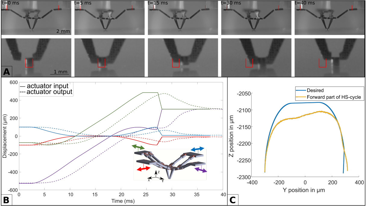
Figure 5: Experimental demonstrations of pick-and-place operations: The manipulated object is a 350\ \mu\text{m} diameter and 400\ \mu\text{m} height silicon cylinder and the result is presented for the forward part of the HS-cycle. A- Motion capture of the manipulator for a pick-and-place HS-cycle. Initial positions of the actuators and the object are represented in red; B- Command vector of each actuator versus the output vector during the forward part of a HS-cycle; C- Trajectory of the end-effectors in the (OYZ) plane for the reference cycle (blue), and HS-cycle (yellow).
