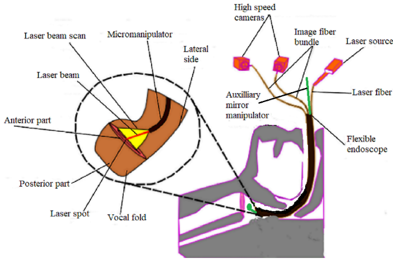
Figure 2. System configuration
