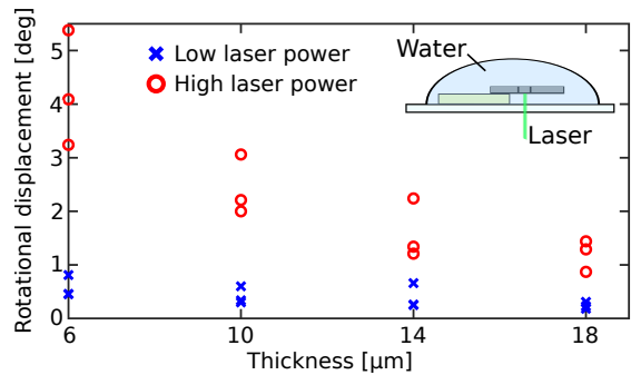
Fig. 7. In water actuation of the microjoint. Blue crosses and red circles show the rotational displacement of the microjoint using low laser power (with ND filters) and using high laser power (without ND filters), respectively. The same sets of three different microjoints were used for low and high laser powers for each thickness.
