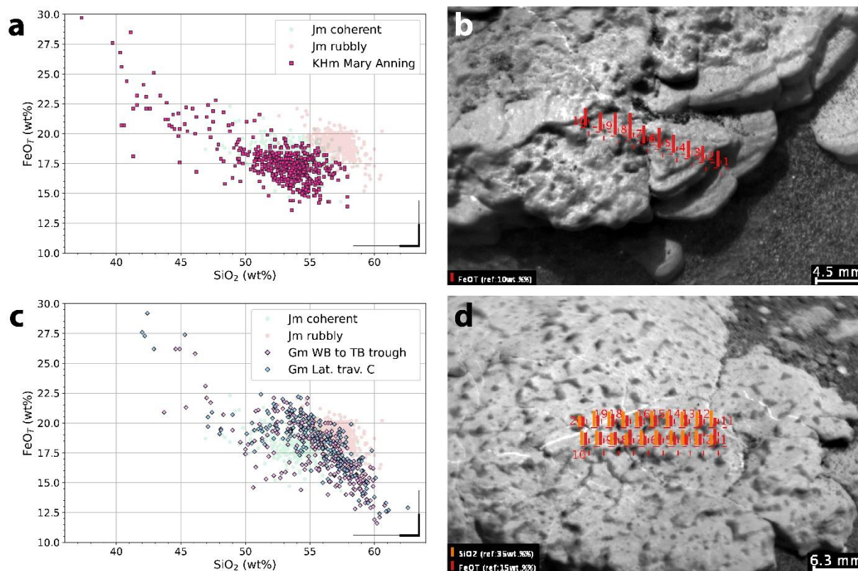
Figure 5. Iron variability observed in the Knockfarril Hill (KHm) and Glasgow (Gm) members. (a) FeO T vs SiO 2 plot for the bedrock of the Mary Anning area. The error bars in the lower right corner represent the accuracy (thin line) and precision (thick line) of the relevant oxides. (b) RMI image of target Formartine (sol 2867), which is located within the knobby-looking layer of the Mary Anning area where high-Fe points were identified. The red bars represent the FeO T abundances of each point of the raster. (c) FeO T vs SiO 2 plot for the bedrock analyzed in two areas of the Glasgow member (Lat. trav. C = Lateral traverse C; TB = Tower butte; WB = Western butte; see figure 1 for localizations). (d) RMI image of target Glenalmond (sol 2656), a bedrock slab with embedded dark-toned features located in the trough between Western butte and Tower butte. The orange and red bars represent the SiO 2 and FeO T abundances of each point of the raster. In the two left panels, Jura coherent and rubbly bedrock compositions are displayed as semi-transparent points for comparison.
