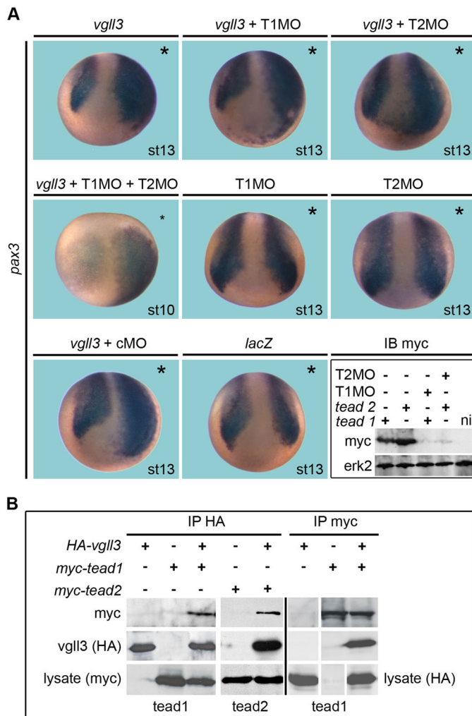
Fig. 7. Vgll3 interacts with tead proteins and can activate pax3 independently of tead. (A) Embryos injected with vgl3 (1 ng or lacZ ) mRNA and T1MO/T2MO or cMO were fixed at stage 10 or 13 and analysed for pax3 . Vgll3 induces ectopic pax3 expression when tead1 and tead2 have been knocked down. Lower right panel (IB myc): embryos were injected with 50 pg myc-tead1 or myc-tead2 mRNAs with 15 ng T1MO or T2MO and analysed by immunoblotting (IB). T1MO and T2MO efficiently block tead1 and tead2 expression, respectively. Erk2 was used as a control. ni, noninjected embryo. (B) Embryos injected with HA- vgl3 , myc-tead1 or myc-tead2 mRNAs were processed for immunoprecipitation with HA (IP HA) or myc antibodies (IP myc) followed by IB with antibodies. Vgll3 interacts with tead1 and tead2 in the embryo. Lysate, IB of injected embryo before immunoprecipitation. Vertical white lines indicate spliced images in order to remove results not described in this paper (IP myc).
