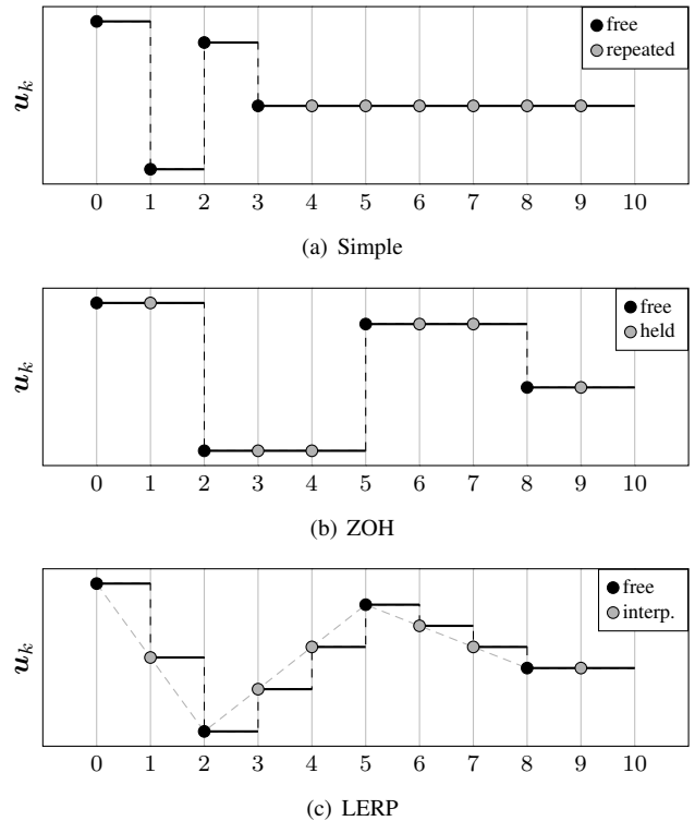
Fig. 1. Example of control sequences \underline{\mathbf{u}} with a reduced number of degrees of freedom. Even if the prediction horizon is N_p = 10 , only 4 variables are freely assigned, while the remaining ones are defined in function of the free samples.
