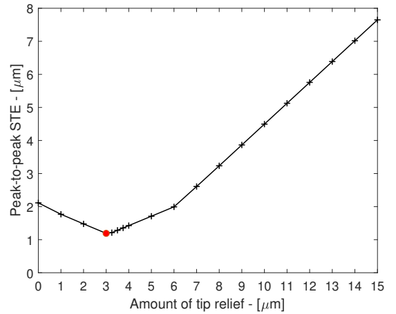
Figure 6: Evolution of the peak-to-peak static transmission error with respect to the amount of tip relief. The red dot denotes the optimum solution, corresponding to the smallest peak-to-peak value of the static transmission error
