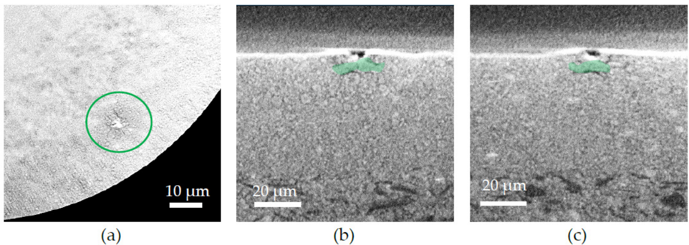
Figure 7. X-ray tomography images of a defect in the upper layers of the raw sample: (a) image from the top (Y-axis) of the defect in the electrolyte; (b) cross-section where the defect is along the X-axis with a NiO grain (in green) in the AFL; (c) cross-section where the defect is along the Z-axis with a NiO grain (in green) in the AFL.
