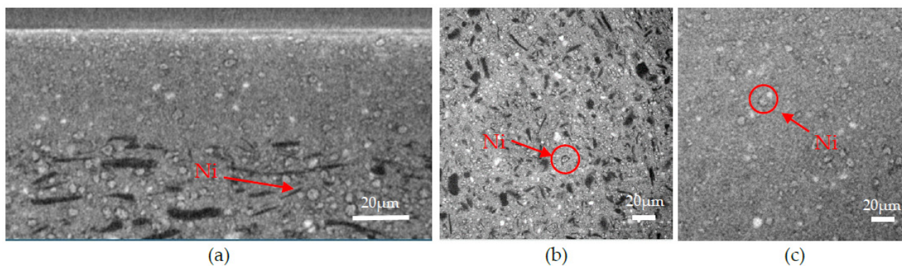
Figure 10. X-ray tomography images of the reduced sample: (a) cross-section along the X-axis; (b) cross-section of the anode along the Y-axis; (c) cross-section of the AFL along the Y-axis.
