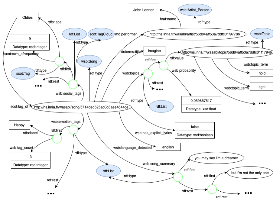
Fig. 18: RDF representation of a song, its artist and some properties related to lyrics analysis. The following namespaces are used: mo : Music Ontology, wsb : WASABI Ontology, scot : SCOT Ontology.).
