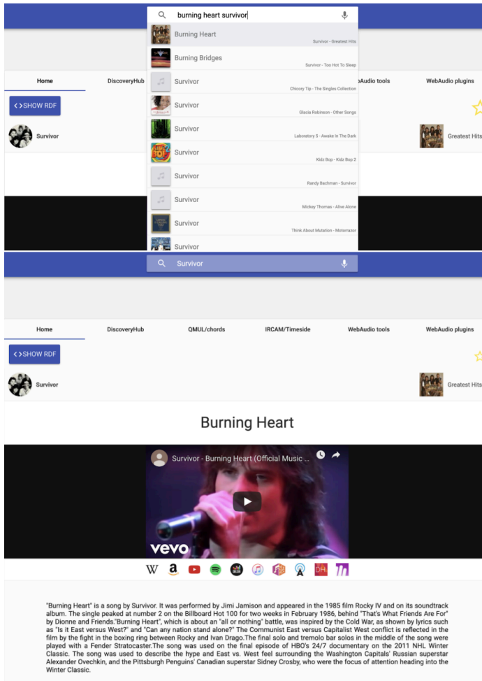
Fig. 1: The WASABI Interactive Navigator [15].
