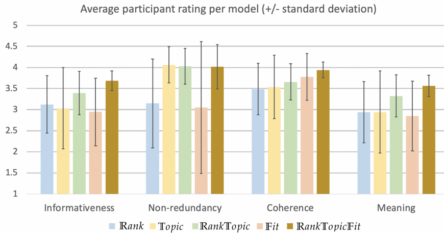
Fig. 5: Human ratings per summarization model (five point Likert scale). Models are \mathbb{R}ank : graph-based, \mathbb{T}opic : topic-based, \mathbb{F}it : thumbnail-based, and model combinations.
