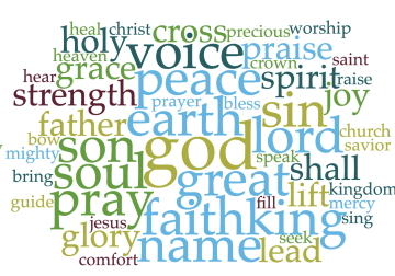
Fig. 13: Topic Religion
