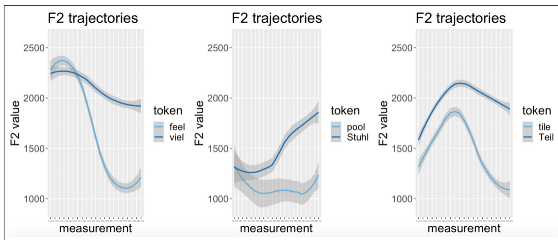
Figure 1: Smoothed F2 trajectories in similar English (light blue) and German (dark blue) words: feel [fi:t̚] versus viel [fi:l] ‘much’ (left); pool [pu:t̚] versus Stuhl [ʃtu:l] ‘chair’ (center); tile [taɪt̚] versus Teil [taɪl] ‘part’ (right). Formant values extracted at 20 equally spaced steps across the vowel-lateral sequence in the acoustic data recorded for the present study.
