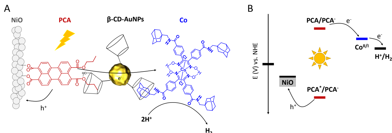
Figure 1. A) Representation of the PCA|β-CD-AuNPs|Co supramolecular assembly anchored onto a mesoporous NiO thin film, B) Energy diagram of the photocathode.
