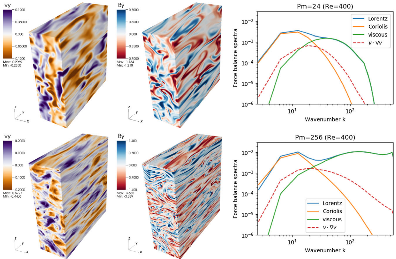
Figure 2. 3D rendering of the azimuthal component of the velocity field (left panels) and of the magnetic field (middle panels). The right-hand panels represent the time-averaged spectra of the force balance. The upper row corresponds to a simulation with a moderate value of Pm = 24 , while the lower row corresponds to a large value of Pm = 256 . Both simulations share the same Reynolds number Re = 400 . In the force balance spectrum, only the divergence-free part of the forces is included as it is appropriate in the incompressible approximation.
