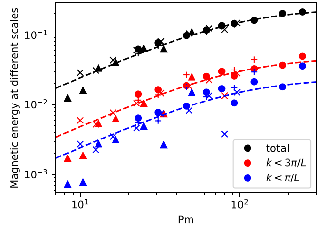
Figure 5. Magnetic energy contained in the largest scales of the box as a function of the magnetic Prandtl number. Blue and red symbols correspond to the energy at wavenumbers smaller than \pi/L and 3\pi/L , respectively, while black symbols show the total magnetic energy. The symbol shapes correspond to different Reynolds numbers as in Fig. 1: Re = 400 (circles), Re = 800 (crosses), and Re = 1600 (triangles). The low resolution tests at Re = 400 are represented with the plus signs. The dashed lines represent the fit of the total magnetic energy (black), and a fraction of 20 per cent (red) and 10 per cent (blue) of this fit, respectively.
