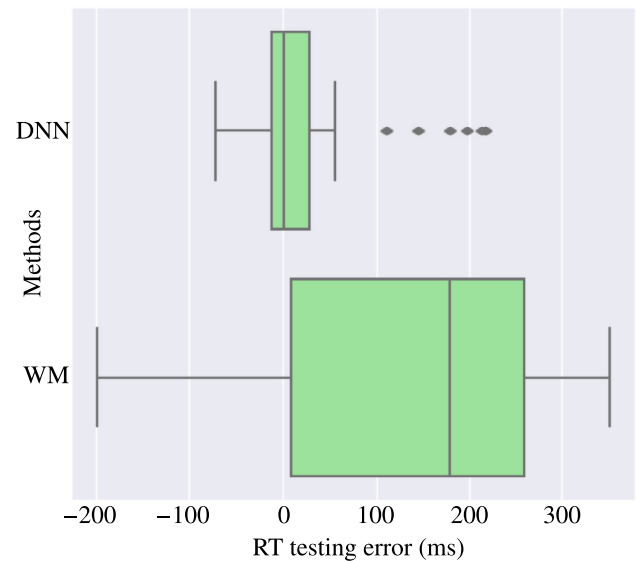
Fig. 5. The distributions of RT estimation errors for the testing ex-vivo UEs when computed using our DNN (absolute error mean = 31.47 ms, median = 16.91 ms, s.d. = 44.59 ms) and the Wyatt method (WM) (absolute error mean = 143.05 ms, median = 182.0 ms, s.d. = 120.25 ms).
