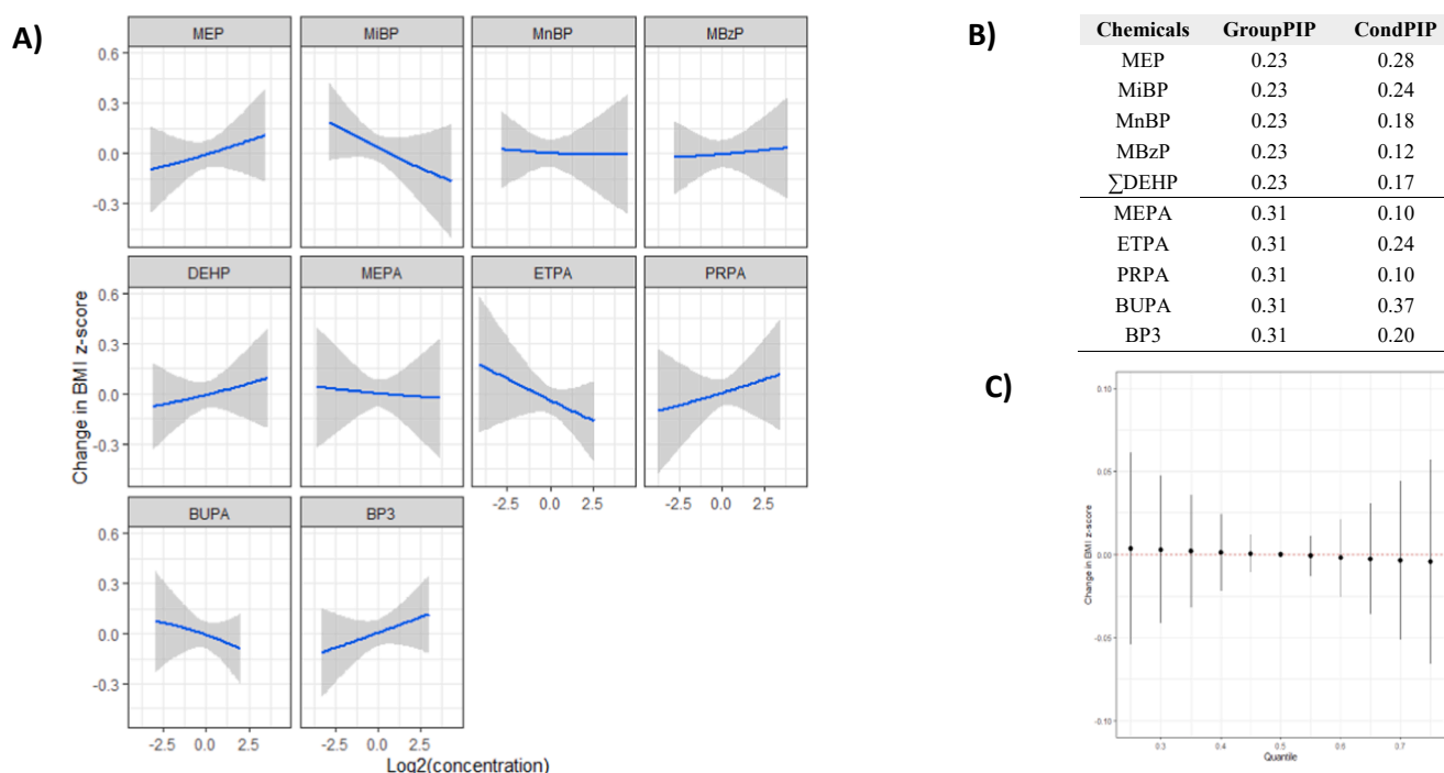
Fig. 3. Summary estimates from BKMR on the association between mixtures of log 2 scaled non-persistent chemicals and BMI z-score in preadolescence adjusted by maternal age, education, smoking in pregnancy and pre-pregnancy BMI; region of residence was included as random intercept. (A) Exposure-response associations for each chemical when the others are fixed at their median. (B) Group and conditional posterior inclusion probabilities (GroupPIP and CondPIP) of each chemical in the mixture-response function for BMI z-score. (C) Joint effect of prenatal non-persistent chemicals mixture on BMI z-score at preadolescence (Credible intervals overlapping the null depicted with the broken line indicate no significant effects). Abbreviations: BMI (body mass index), BKMR (Bayesian kernel machine regression), MEP (mono-ethyl phthalate), MiBP (mono-iso-butyl phthalate), MnBP (mono-n-butyl phthalate), MBzP (mono-benzyl phthalate), DEHP (sum di(2-ethylhexyl) phthalate metabolites), MEPA (methyl paraben), ETPA (ethyl paraben), PRPA (propyl paraben), BUPA (butyl paraben), BP3 (benzophenone-3).
