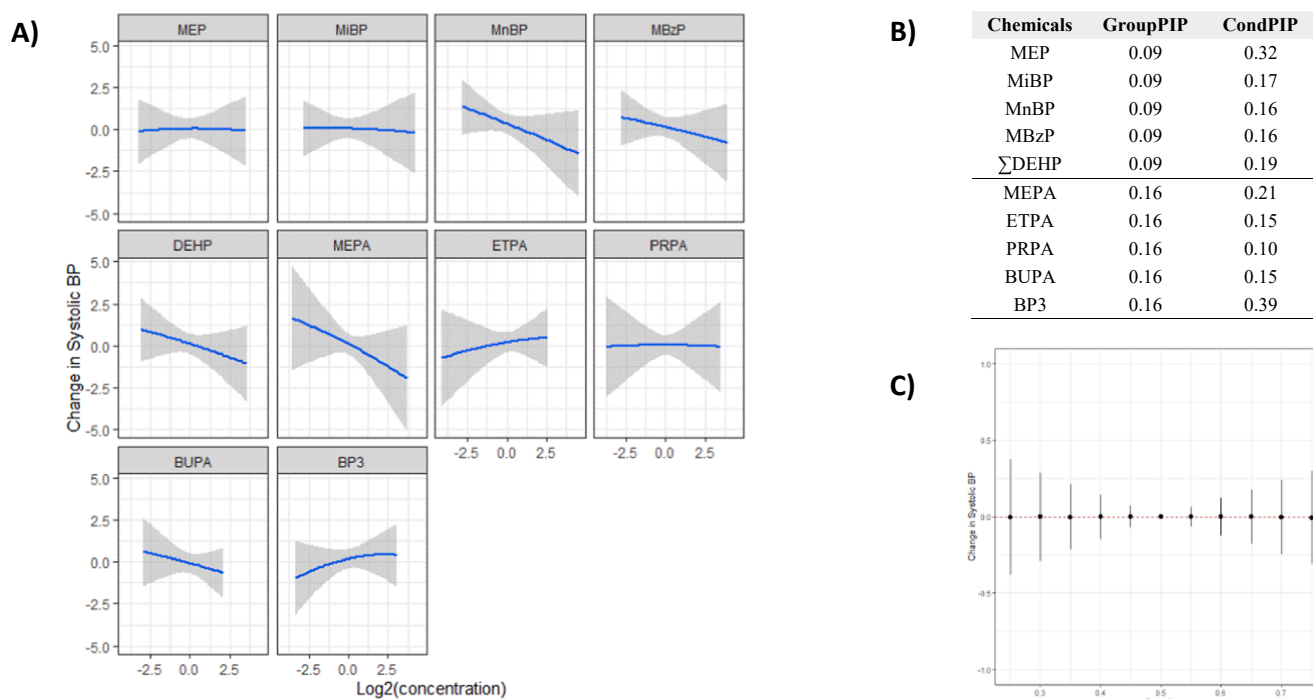
Fig. 4. Summary estimates from BKMR on the association between mixtures of log 2 scaled non-persistent chemicals and systolic BP in preadolescence adjusted by maternal age, education, smoking in pregnancy, pre-pregnancy BMI, sex, height and age at outcome assessment; region of residence was included as random intercept. (A) Exposure-response associations for each chemical when the others are fixed at their median. (B) Group and conditional posterior inclusion probabilities (GroupPIP and CondPIP) of each chemical in the mixture-response function for systolic BP. (C) Joint effect of prenatal non-persistent chemicals mixture on systolic BP at preadolescence (Credible intervals overlapping the null depicted with the broken line indicate no significant effects). Abbreviations: BP (blood pressure), BMI (body mass index), BKMR (Bayesian kernel machine regression), MEP (mono-ethyl phthalate), MiBP (mono-iso-butyl phthalate), MnBP (mono-n-butyl phthalate), MBzP (mono-benzyl phthalate), DEHP (sum of di(2-ethylhexyl) phthalate metabolites), MEPA (methyl paraben), ETPA (ethyl paraben), PRPA (propyl paraben), BUPA (butyl paraben), BP3 (benzophenone-3).
