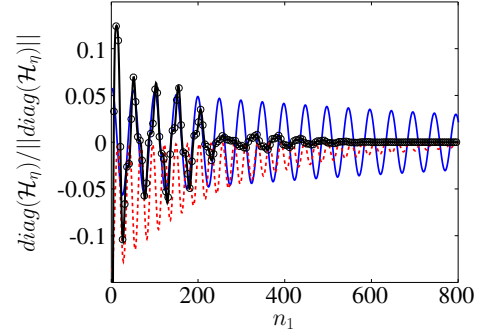
(b) Main diagonal of the Volterra kernels, — is the normalized 1 st kernel, while - - - and - o - are the normalized main diagonal of the 2 nd and 3 rd kernel respectively.
