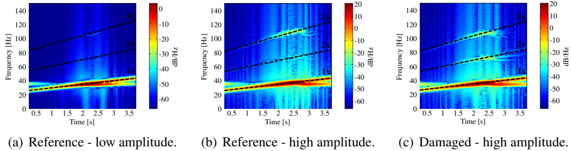
Figure 2: Time-frequency diagram of the system's output exemplifying the presence of nonlinear phenomena.
