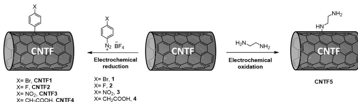
Scheme 1. Electrochemical immobilisation of aryl diazonium salts on the CNTF surface. It is worth noting that chemical representation of CNTFs is depicted as a single carbon nanotube to better illustrate the chemical reactions without reference to the relative sizes of the carbon nanotube and CNTFs.
