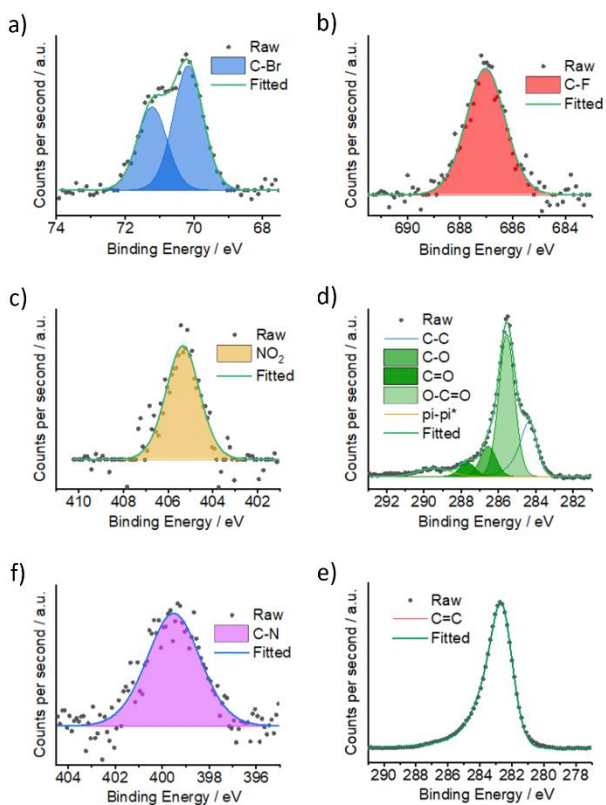
Figure 4. High resolution XPS spectra of functionalised a) CNTF1, b) CNTF2, c) CNTF3, d) CNTF4, e) pristine CNTF, and f) CNTF5 showing Br 2p, F 1s, N 1s, C 1s, C 1s, N1s core levels, respectively. It should be noted that the small diameter of CNTFs (~20 \mu\text{m} ) makes it difficult to obtain an optimal signal-to-noise ratio.
