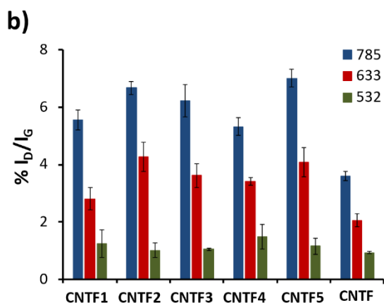
Figure 3. a) Raman average spectra of pristine CNTFs and functionalised CNTFs at 785 nm from line mapping mode of 180 points analysis, with time exposure of 1 s, and 10% power. Inset: optical image of a typical CNTF with the mapping points analysed (from red to black as intensity colour scale), and b) I_D/I_G measured using the different laser sources.
