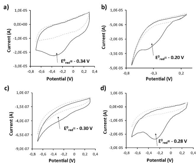
Figure 2. Cyclic voltammogram corresponding to different diazonium salt reduction using 100 mV·s -1 as scan rate. First scan (solid line) shows the reduction of the salt, and second scan (dashed line) shows the absence of an active electrochemical surface for further reduction. The panels correspond to the different aryl diazonium salts CNTF1 (a), CNTF2 (b), CNTF3 (c) and CNTF4 (d), respectively.
