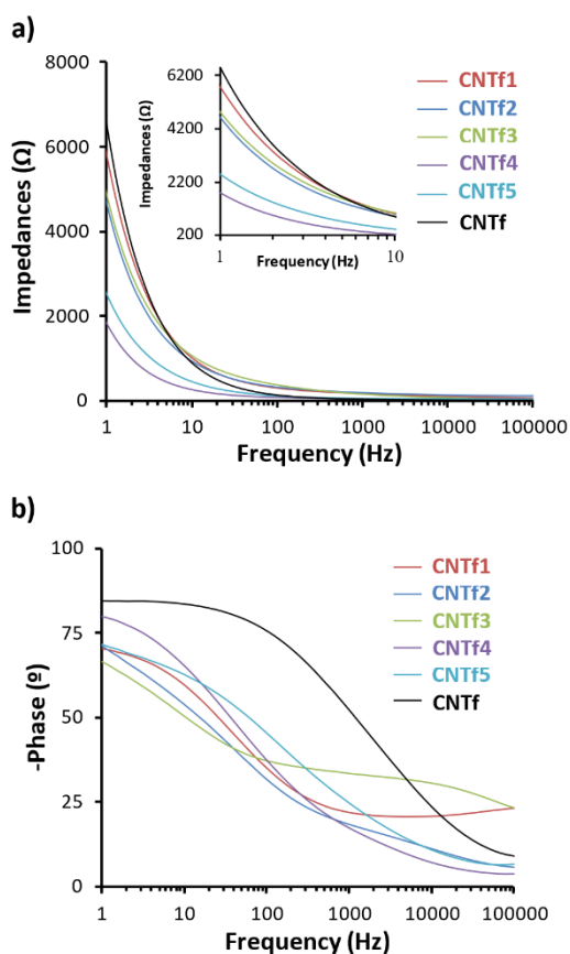
Figure 5. EIS measurement of (a) relative impedance, inset: expanded area from 1 to 10 Hz, and (b) measurements of functionalised CNTFs in PBS (pH=7.4, 0.1 M).
