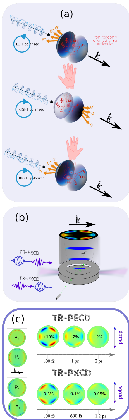
Figure 3 TR-PECD and TR-PXECD appear both as an photoelectron asymmetry relative to the light propagation axis on the velocity map imaging spectrometer (VMIS) image. This asymmetry depends both on the handedness of the molecule and the helicity of the light, as any other chiroptical effect. (b) This asymmetry is monitored with a velocity map imaging detector. In TR-PECD, the probe has to be circularly polarized, while in TR-PXECD, it is the pump that is circularly polarized. (c) The asymmetry images can be fitted by a linear combination of the P_{l=1,3} Legendre Polynomials (as shown in the column at left). Here are shown images of photoelectron asymmetry recorded in TR-PECD and TR-PXECD for different pump-probe delays in the enantiopure 1R,4R-(+)-camphor. Pump-probe ionization takes place at \sim 9.3 eV with a pump excitation in the first Rydberg states of camphor. The colormap is the same for all the delays in each configuration. The indicated percentages correspond to the asymmetry of forward hemisphere recorded with a left polarized probe (TR-PECD) or pump (TR-PXECD). These data have been published in 58 and 59 .
