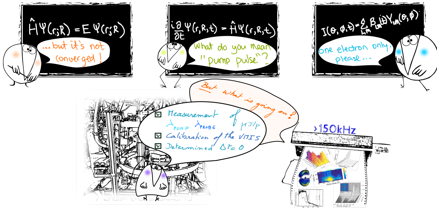
Figure 2 A Shadoks' view of Time-Resolved Photoelectron Spectroscopy for new users : A joint analysis of experimental and theoretical data leads to a quantitative interpretation of the photodynamics.
