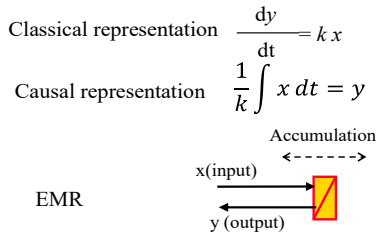
Fig. 4 From classical representation to EMR
