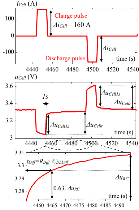
Fig. 11 Characterization pulses
