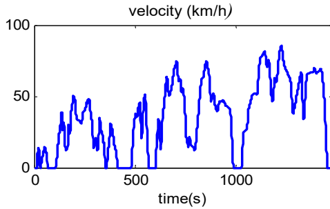
Fig. 18 WLTC driving cycle
