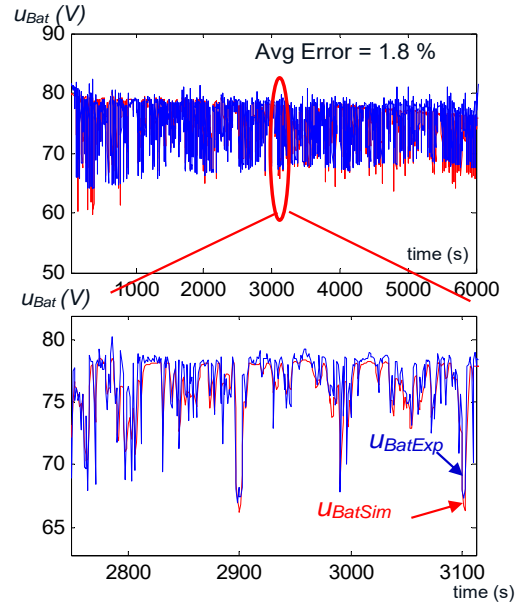
Fig. 17 Experimental and simulated battery voltage
