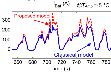
Fig. 19 Battery current at -5°C
