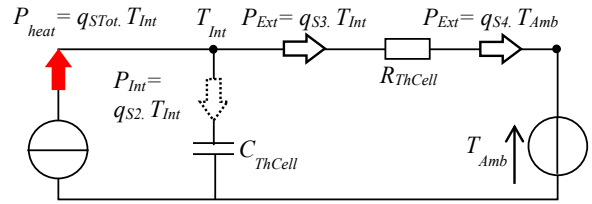
Fig. 6 Flow and effort variables for thermal model [21]
