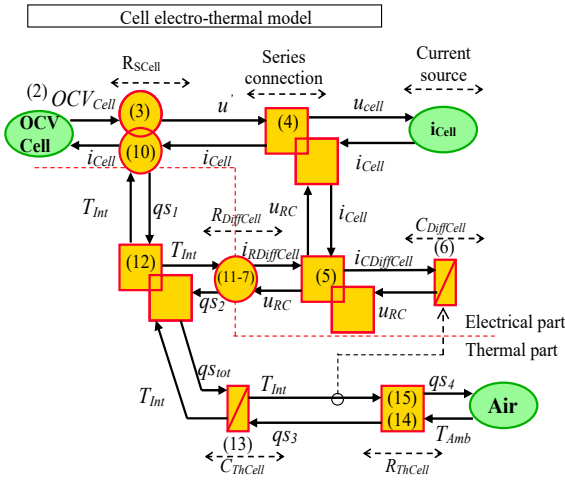
Fig. 5 EMR of the dynamical electro-thermal model[21]
