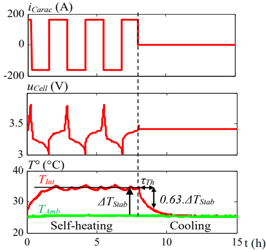
Fig. 13 Thermal characterization protocol
