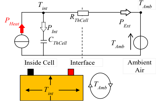
Fig. 2 Structure of the thermal model for one cell [21]
