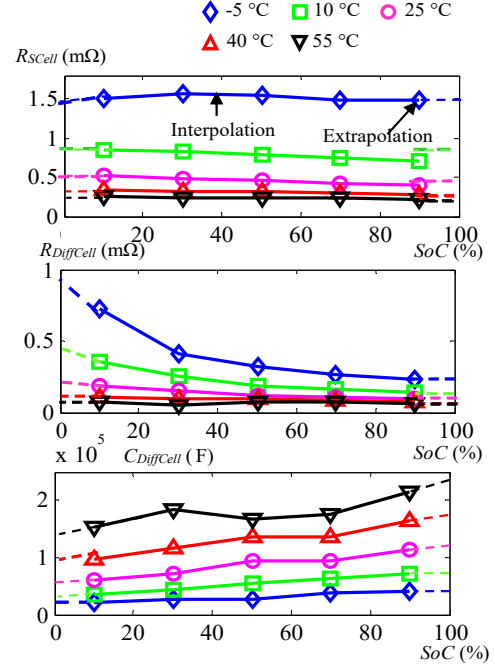
Fig. 12 Impedance parameters with SoC and temperature
