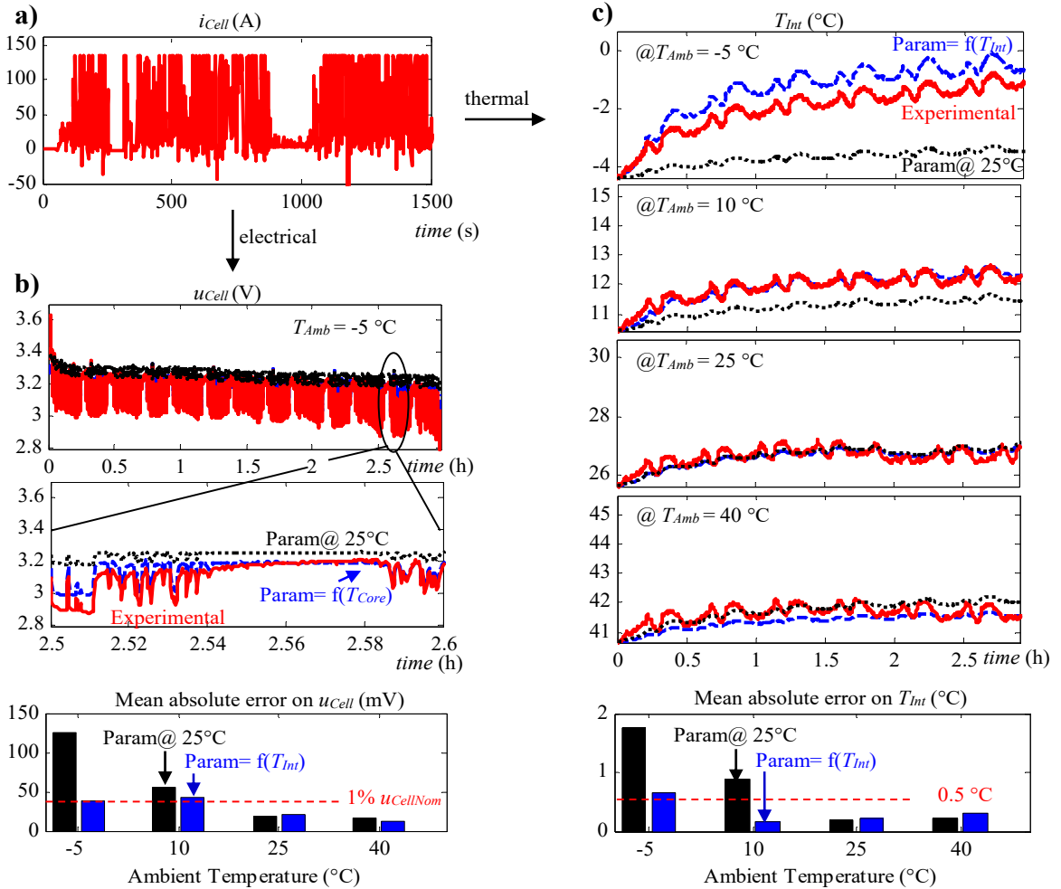
Fig. 14 Real EV current (a) used for electrical (b) and thermal (c) validations of cell model
