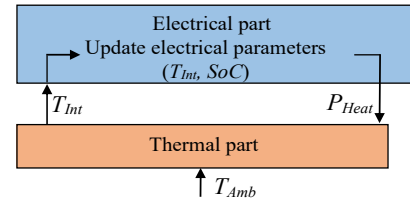
Fig. 3 Electro-thermal coupling principle
