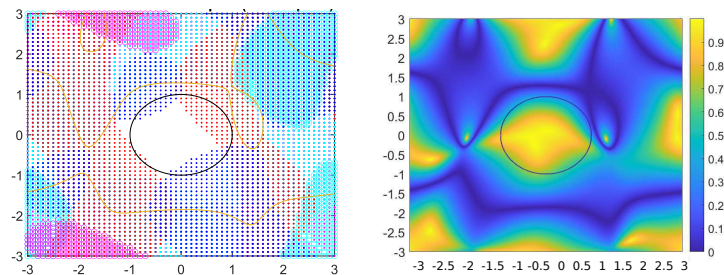
FIGURE 8 – Feasible workspace and heatmap for the quality index with center biased rewarding strategy
