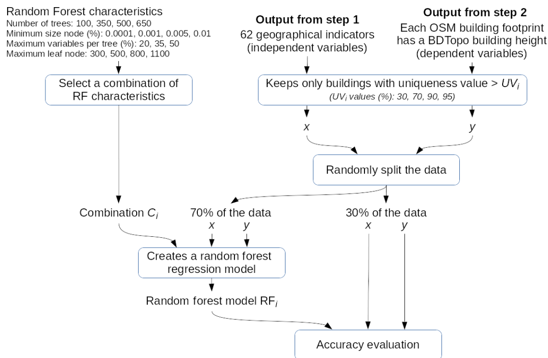
Figure 5. Method to train and optimize the random forest model. Only the training dataset is used at this step.
