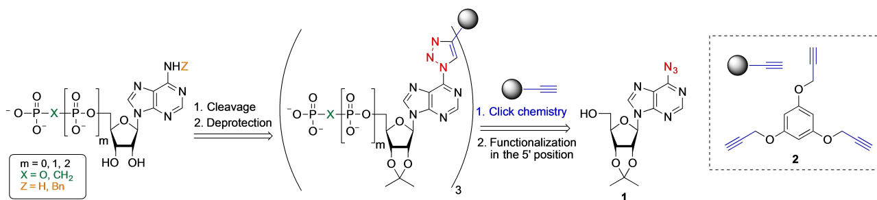
Scheme 1. Retrosynthetic strategy for the synthesis of nucleotides and derivatives.
