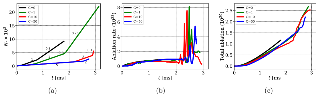
Figure 9: Comparison of the simulations of Neon SPI in JET-like plasma without and with numerical stabilization. The following quantities are plotted vs t [ms] (a) The number of time steps ( N_t ) taken by the simulations. The labels to the curves are the values of the time step \Delta t_* written in the normalized units for the sake of the presentation. The scale to convert \Delta t_* in ms is = 2.973 \times 10^{-4} and hence \Delta t = \Delta t_* \times 2.97 \times 10^{-4} ms. (b) The ablation rate. (c) The total number of impurity atoms ablated in the plasma.
