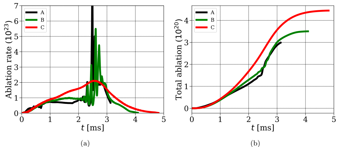
Figure 15: Evolution of a) the ablation rate and b) the total number of impurity atoms ablated in the plasma during Neon SPI simulations in JET-like plasma with different resistivities and shock-capturing coefficient c^{\parallel} = c^{\perp} = c .
