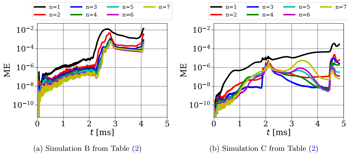
Figure 19: Evolution of the magnetic energies in each toroidal harmonic during neon SPI simulations in JET-like plasma with different resistivities and shock-capturing coefficient c^{\parallel} = c^{\perp} = c .
