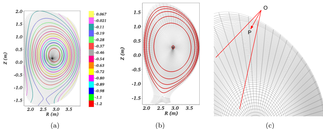
Figure 3: a) The contours for the numerical solution of GSE plotted on the top of the polar grid used. The solution field shows one minimum and one saddle point where \psi = 0 . b) Multi-block grid with grid lines of the each block is aligned to the numerical solution of GSE. Red contours denote the surfaces where safety factor q takes rational values equal to 1 to 7 (radially outwards). (c) A schematic of SPI into JET-like plasma: JOREK grid denoting JET-like computational domain. The SPI fragments are shattered into a curved tube before releasing into the tokamak plasma. The red lines show the cone in which SPI fragments travel in the tokamak plasma.
