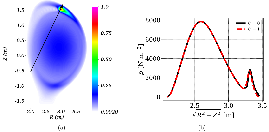
Figure 7: Numerical results axisymmetric source term modeling argon SPI in JET-like plasma computed with different shock-capturing stabilization coefficient c = c^{\parallel} = c^{\perp} . (a) The particle density n_f [ 10^{20} ] plotted at \phi = 0 plane and t \approx 0.562 ms. The line is traced approximately along the direction of SPI velocity and passing through the location of the source term. (b) The pressure plotted along this line at the same time instant.
