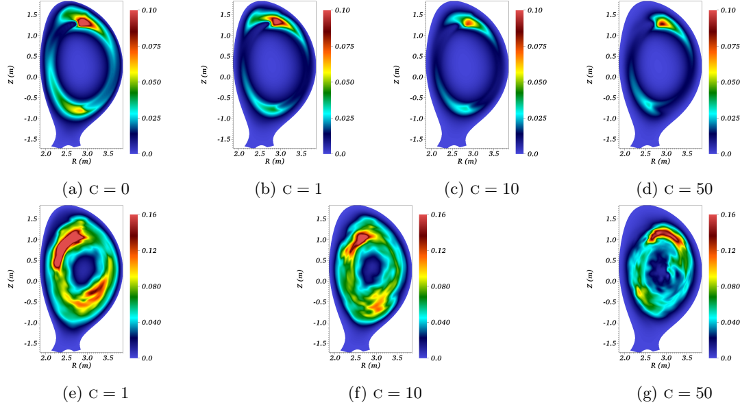
Figure 11: Snapshots of the impurity particle density n_f [10^{20} \text{ m}^{-3}] plotted in the poloidal plane \phi = 0 with the shock-capturing stabilization coefficient c^{\parallel} = c^{\perp} = c . Top and bottom rows show visualization at t \approx 1.6 and 2.73 ms respectively.
