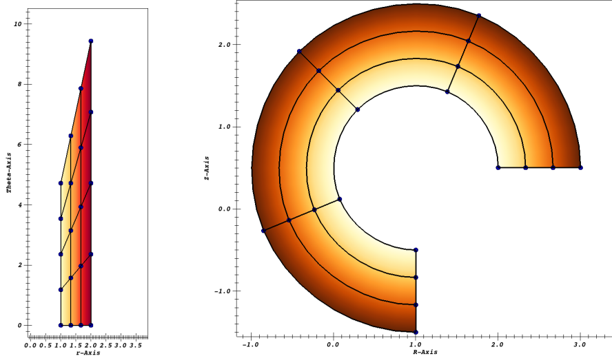
Figure 1: An example of annular mesh in the parametric (left) and in the physical (right) spaces. The color map in both cases denotes the values of the small radius ( r ).
