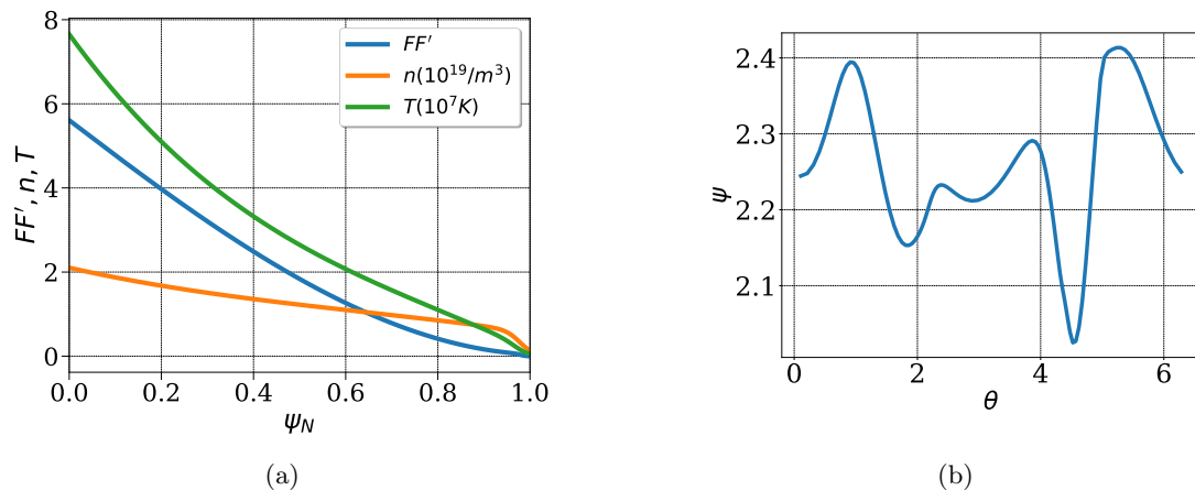
Figure 2: JET-like plasma equilibrium : (a) The profiles characterising plasma equilibrium b) boundary conditions on \psi to be specified for a polar grid plotted vs azimuthal direction \theta .
