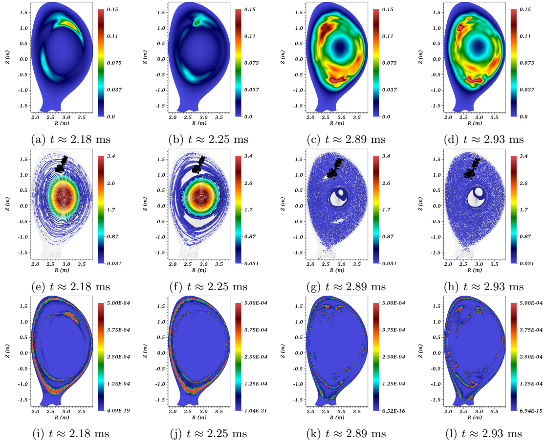
Figure 13: Snapshots of the impurity particle density n_f [10 20 ] (first line), Poincaré plots of the magnetic field (second line), and the shock-capturing parameter \tau_{sc} (last line) at the mentioned time instants. The figures in the first and second lines are plotted in the poloidal plane \phi = 0 . The black dots in the figures with Poincaré plots denote the positions (projected onto the poloidal plane) of the SPI fragments while the color denotes values of the plasma temperature in keV. These visualizations are from the simulation with the shock-capturing stabilization coefficient c^{\parallel} = c^{\perp} = c = 10 .
