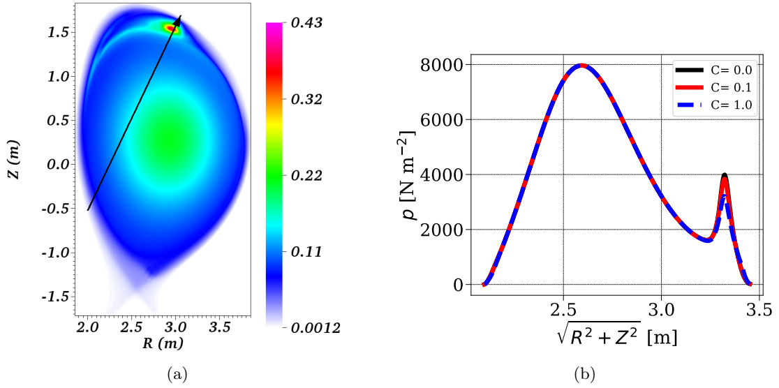
Figure 5: Numerical results axisymmetric source term modeling argon SPI in JET-like plasma computed with different shock-capturing stabilization coefficient c^{\parallel} = c^{\perp} = c . (a) The total particle density n_0 [ 10^{20} ] plotted at \phi = 0 plane and t \approx 0.562 ms. The line is traced approximately along the direction of SPI velocity and passing through the location of the source term. (b) The pressure plotted along this line at the same time instant.
