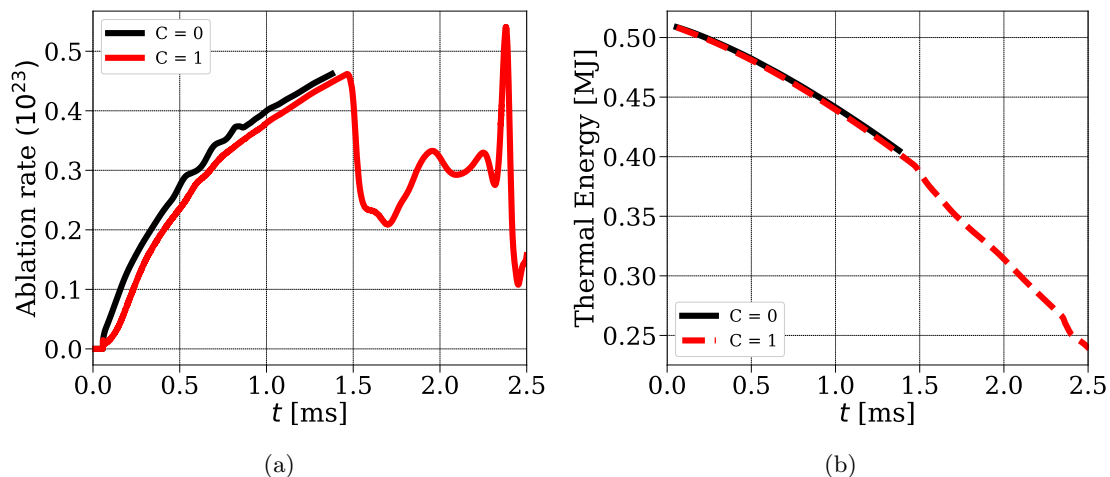
Figure 6: Numerical results for the axisymmetric source term modeling of argon SPI in JET-like plasma computed with different shock-capturing stabilization coefficient c = c^{\parallel} = c^{\perp} . Evolution of (a) ablation rates (b) thermal energies for argon SPI simulations with the axisymmetric source.
