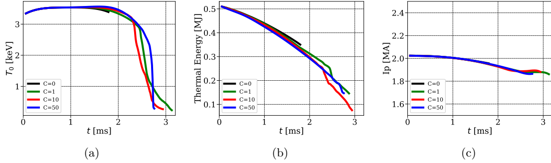
Figure 14: Evolution of the (a) plasma temperature at the magnetic axis [keV] (b) plasma thermal energy [MJ] and (c) plasma current I_p [MA].
