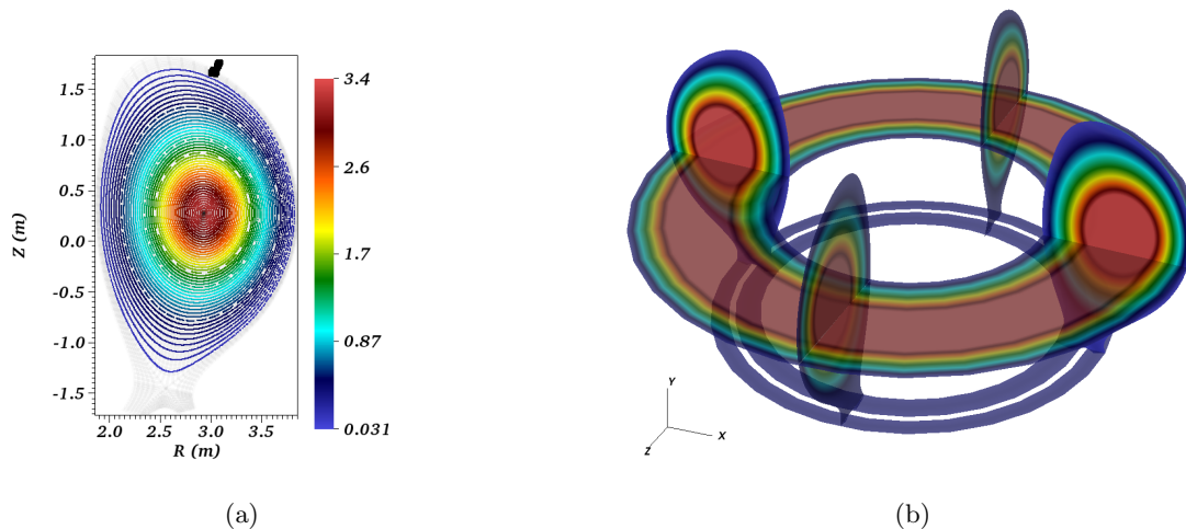
Figure 8: (a) At the beginning of SPI simulations some fragments (denoted by black dots) are spatially distributed (they may even be outside the plasma). The colors of the contours denote the magnitude of T in keV. (b) 3D temperature field at the beginning of the simulation showing axisymmetry.
