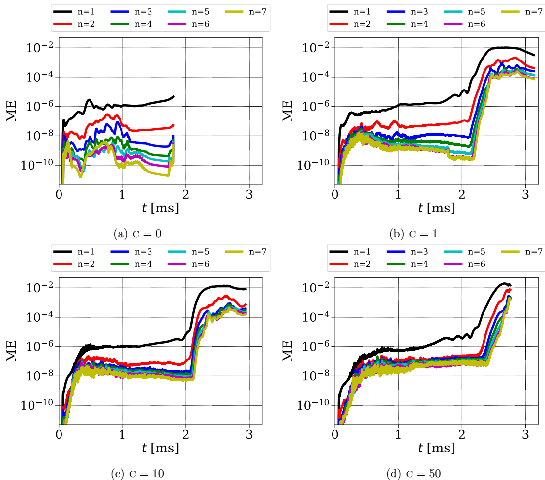
Figure 10: Evolution of the magnetic energies in each toroidal harmonic in the SPI simulation with \eta_0 = 4.22 \times 10^{-8} [Ohm.m] and c^{\parallel} = c^{\perp} = c .
