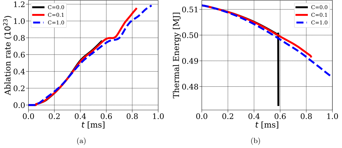
Figure 4: Numerical results axisymmetric source term modeling argon SPI in JET-like plasma computed with different shock-capturing stabilization coefficient c^{\parallel} = c^{\perp} = c . Evolution of (a) ablation rates (b) thermal energies for argon SPI simulations with the axisymmetric source.
