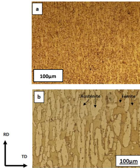
Fig. 2 Microstructure of the dissimilar steels (a): X70 steel, and (b): duplex stainless steel.
