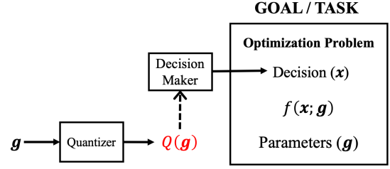
Fig. 1: Proposed definition for the goal-oriented quantization approach
