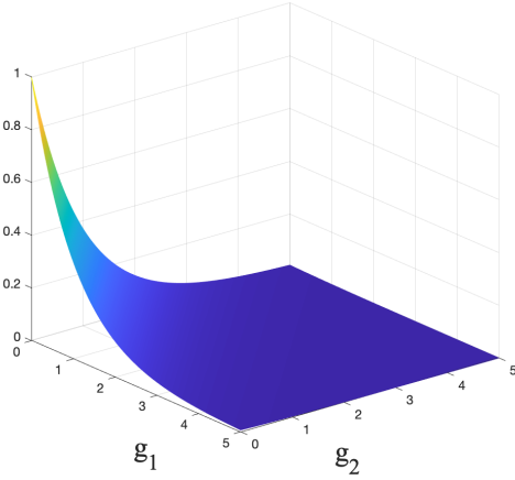
(b) Original probability distribution \phi(g)
