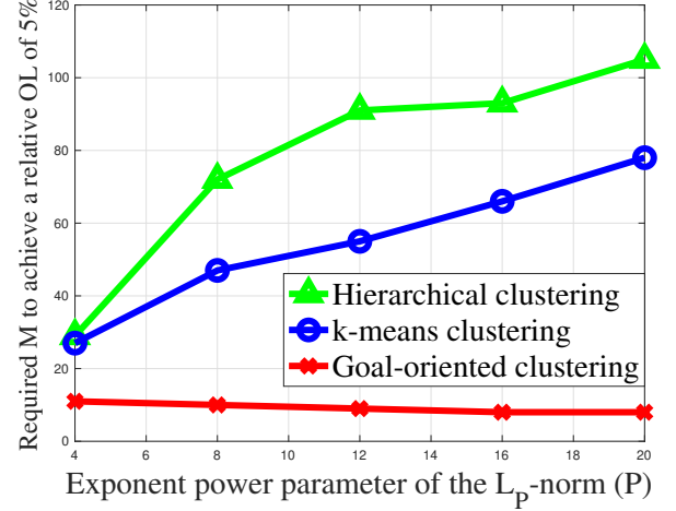
Fig. 6: Required number of clusters ( M ) against the Exponent power parameter of the L_P -norm ( P ) for the k -means and goal-oriented clustering. The goal-oriented clustering approach yields a drastic reduction in terms of the number of clusters when P increases.
