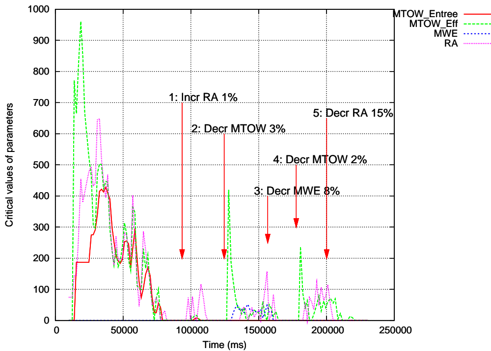
Figure 9: Critical values of parameters RA , MTOW and MWE
