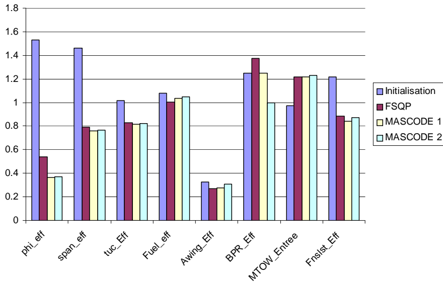
Figure 4: Comparison of input objectives obtained with FSQP and Mascode.
