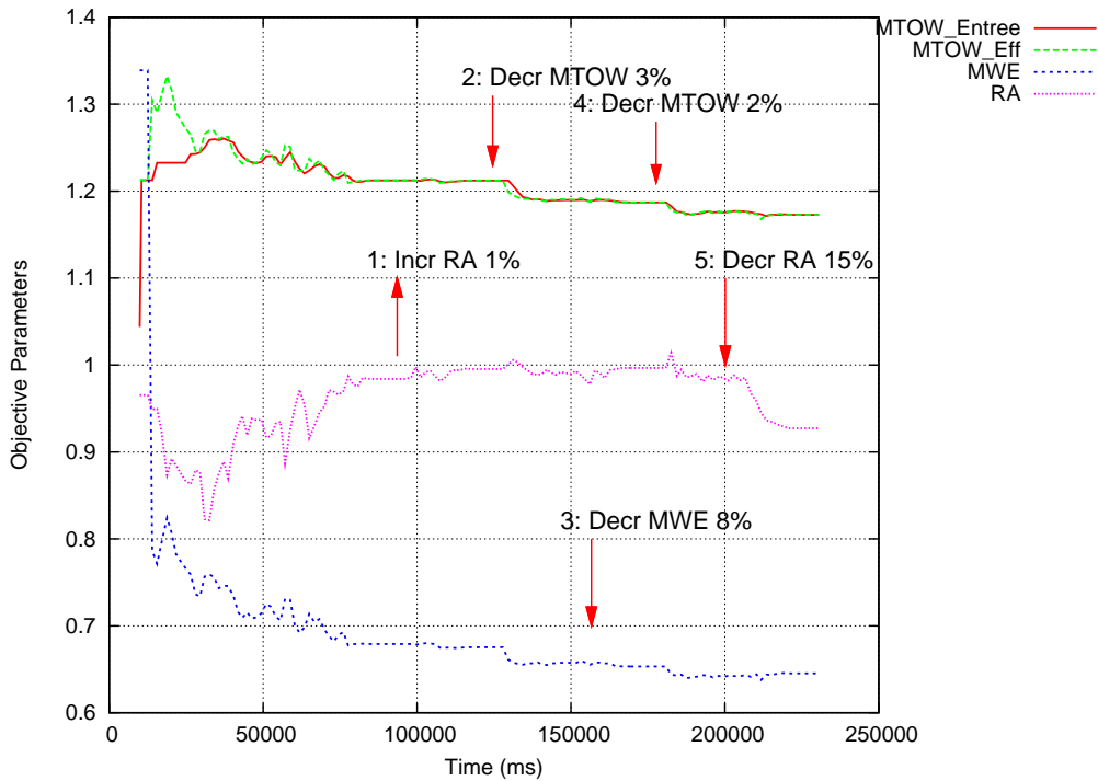
Figure 8: Values of parameters RA , MTOW and MWE
