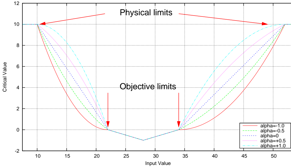
Figure 2: Evaluation functions of critical values (interval validity functions).
