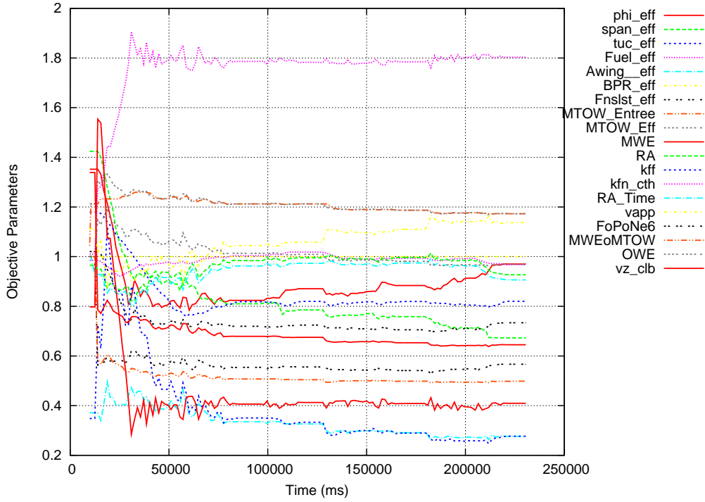
Figure 6: Evolution of objective parameters during a Mascode execution
