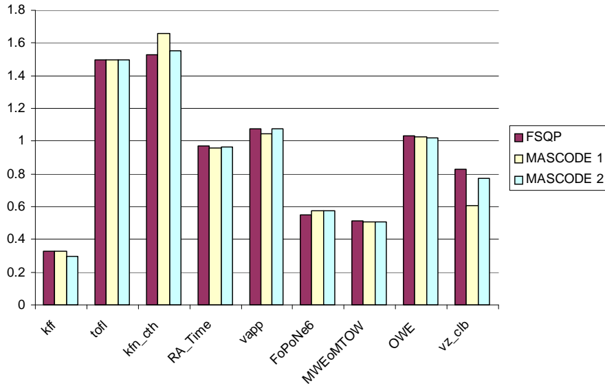
Figure 5: Comparison of output objectives obtained with FSQP and Mascode.
