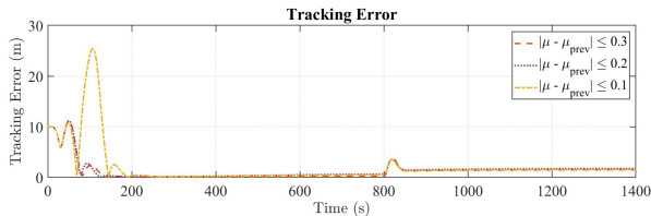
Fig. 10. Tracking error results varying input increment constraints.
