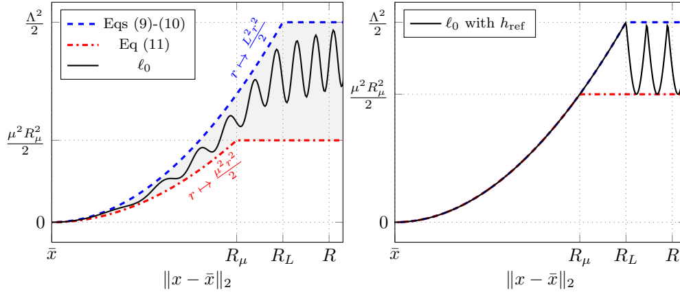
Figure 3: Left : Illustration of quantities \Lambda , L , \mu and R_\mu . The noiseless cost function \ell_0 is sandwiched between two quadratic functions near \bar{x} and between two constants far away from the origin. Right : The specific case h_{\text{ref}} where \mu = L .
