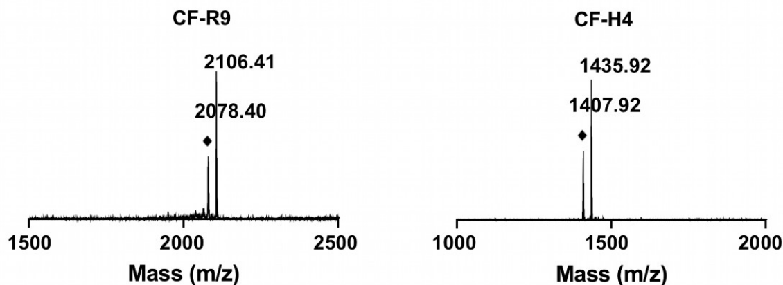
Figure 2. a) Synthesis of the azidopeptides CF-R9 and CF-H4 . Note that the peptides have a carboxamide function at their C-terminus. Pep = peptide, CF = 5(6)-carboxyfluorescein. b) MALDI-TOF mass spectra of CF-R9 and CF-H4 . Peaks labelled by ♦ correspond to a loss of 28 compared to the expected m/z values, presumably due to the expulsion of N 2 during MALDI-TOF MS analysis.
