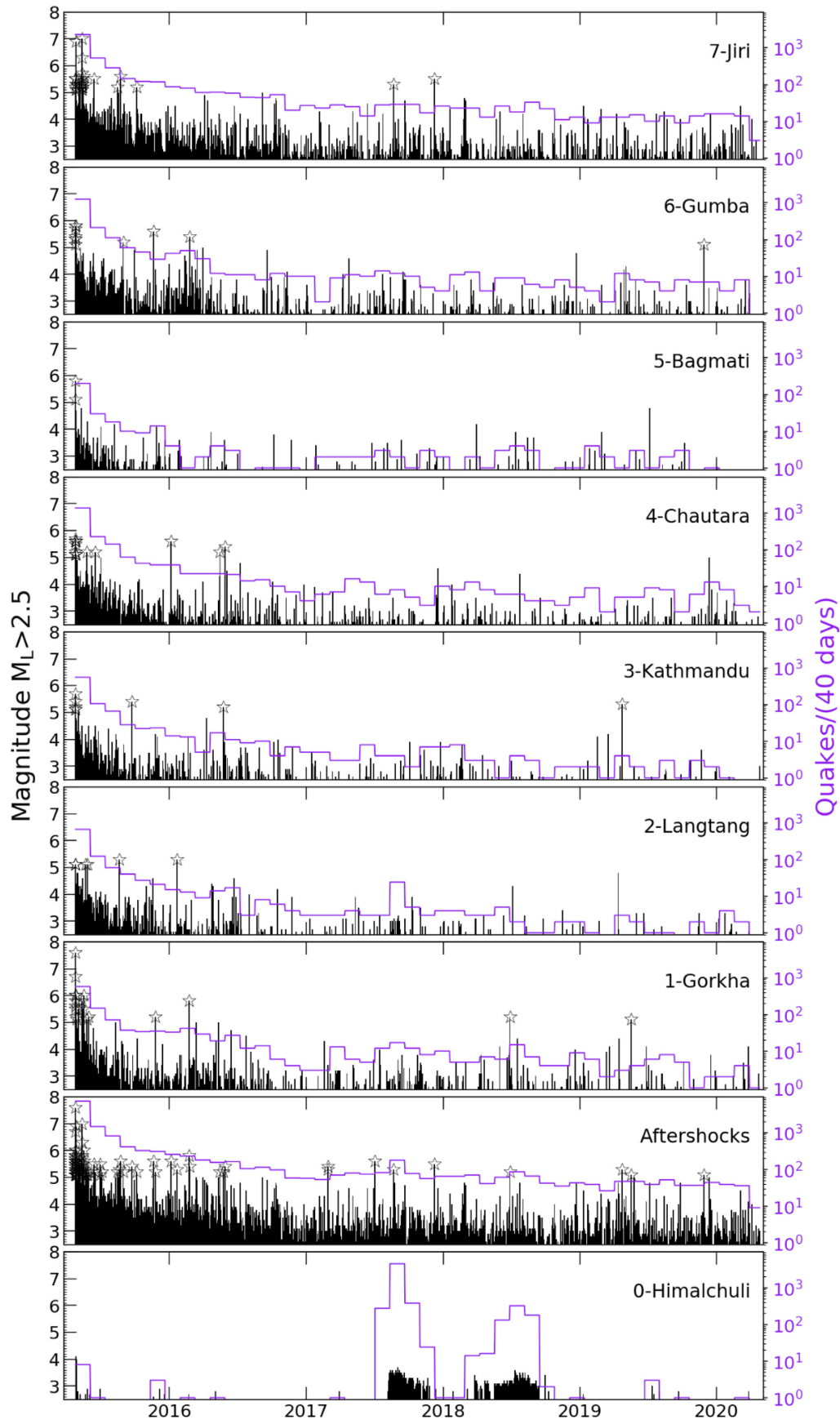
Figure 10. Time structure of the seismicity since the main shock in every zone (defined in Fig. 6). The histograms refer to the number of events per period of 40 d with the scale given to the right.
