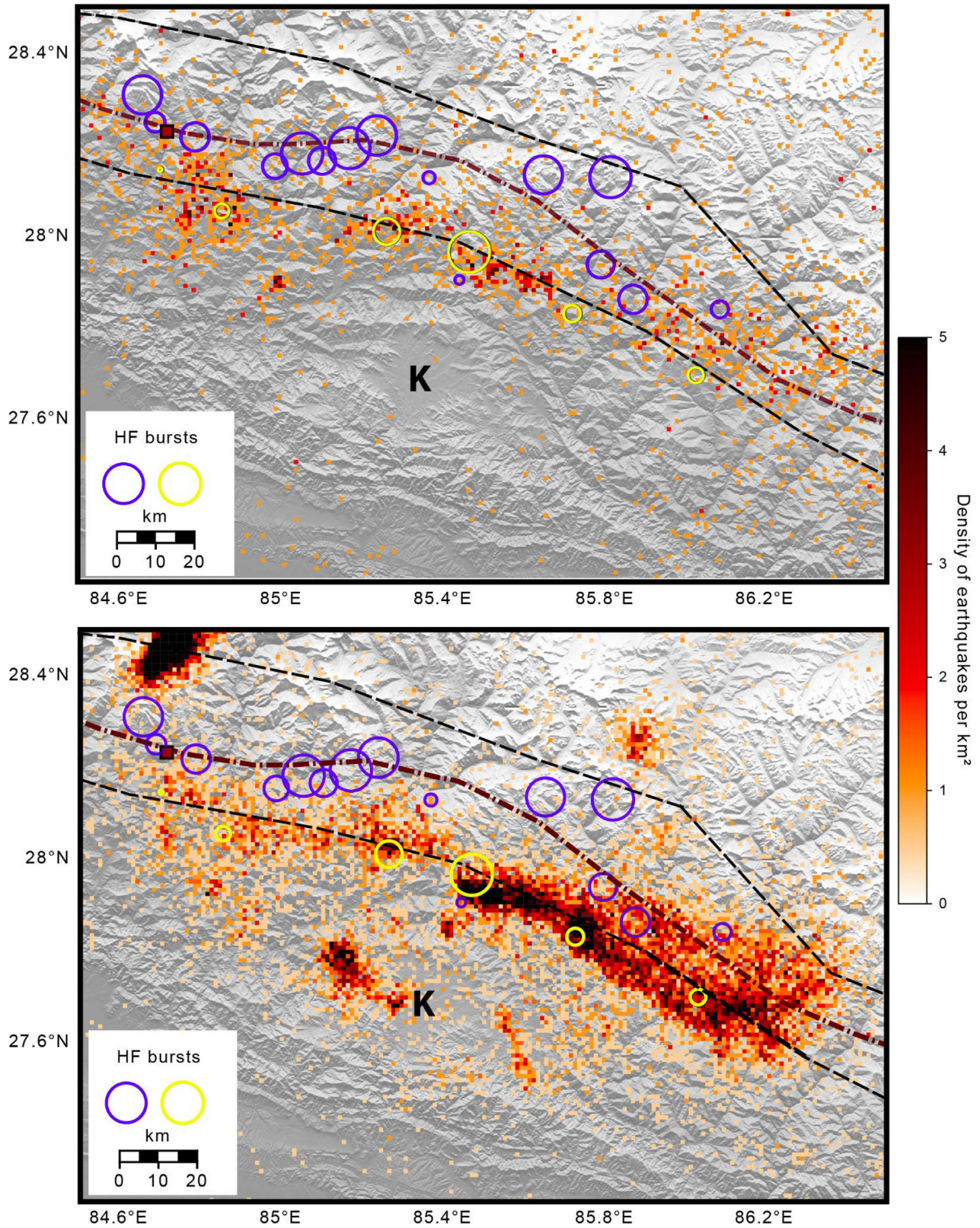
Figure 13. Confrontation between (a) the density of seismicity during the interseismic period (1994–2014) and (b) the density of aftershocks after the 2015 April 25 M_w 7.9 Gorkha earthquake. Density of earthquakes is computed as the log normalized of the number of events greater than M_L 2.5 per \text{km}^2 . Brown dot-dashed line is the geologically inferred location of the base of the mid-crustal ramp (Hubbard et al. 2016). Black dashed lines correspond to the 95 per cent confidence range for the downdip extent of the coupling from Lindsey et al. (2018). Yellow circles are the high-frequency (0.5–4 Hz) peaks inferred from the backprojection of teleseismic P waves during the Gorkha rupture (Qin & Yao 2017). Blue circles are the high-frequency (1–4 Hz) peaks inferred from the backprojection of teleseismic P waves during the Gorkha rupture (Grandin et al. 2015). Size of circles depends on the normalized peak energy. Peaks locations depend on the relative location of the hypocentre. K, Kathmandu.
