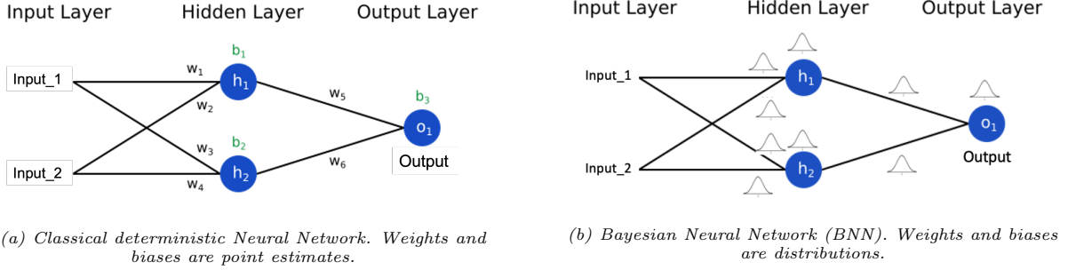
Figure 1: Comparing a standard neural network to a BNN.
