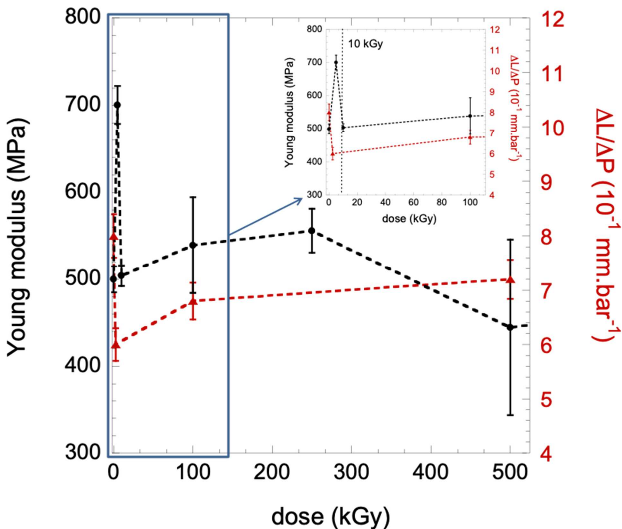
Figure 9: comparison between Young's modulus variations and deformation induced by pressure with the dose; inset: mirror effect in the low dose range with strong variation of Young's modulus and corresponding polymer displacement with pressure.
