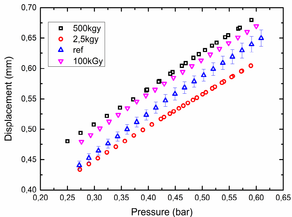
Figure 8: measured displacement of PVDF films plotted against the applied pressure in the experimental cell used for piezoelectric response registration
