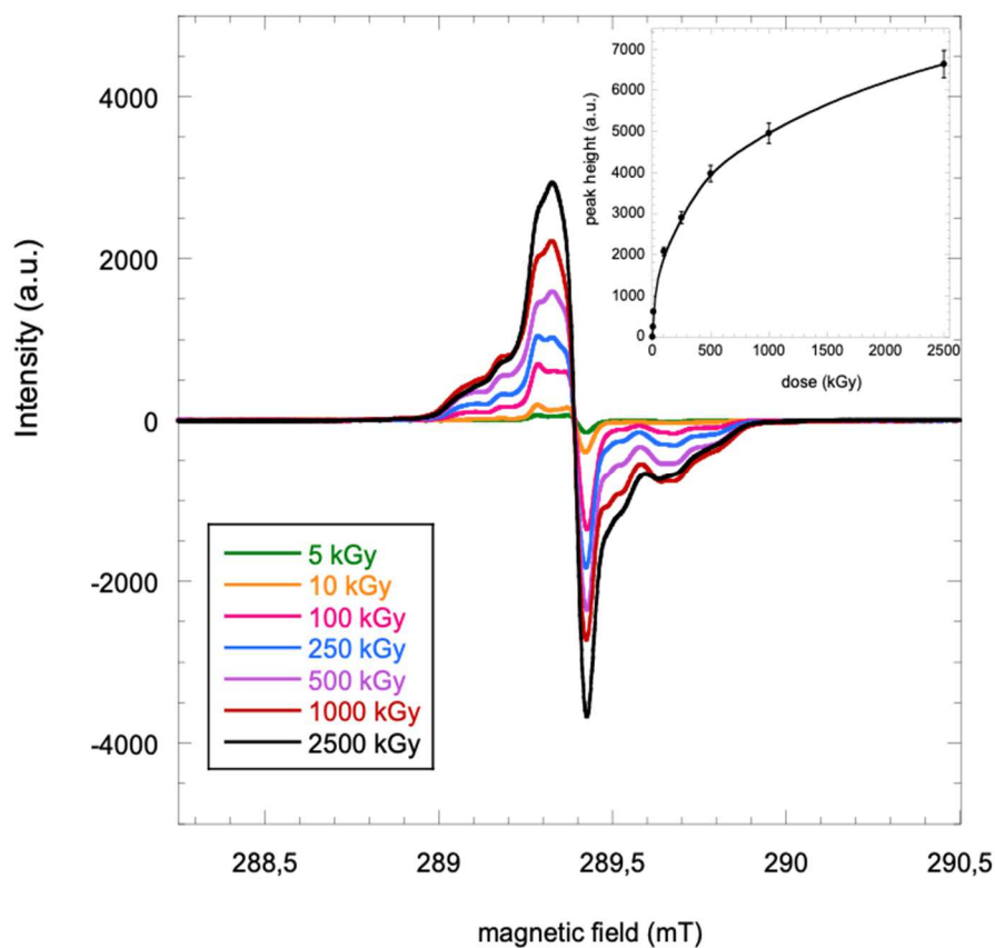
Figure 5: EPR spectra of e-beam irradiated piezoPVDF films at various doses; inset: peak height versus dose
