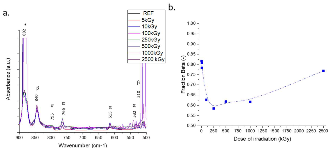
Figure 7: a. Comparison with FT-IR spectra of irradiated PVDF polymer in dose range of 5-2500 kGy and reference sample, b. \beta fraction as function of irradiation dose
