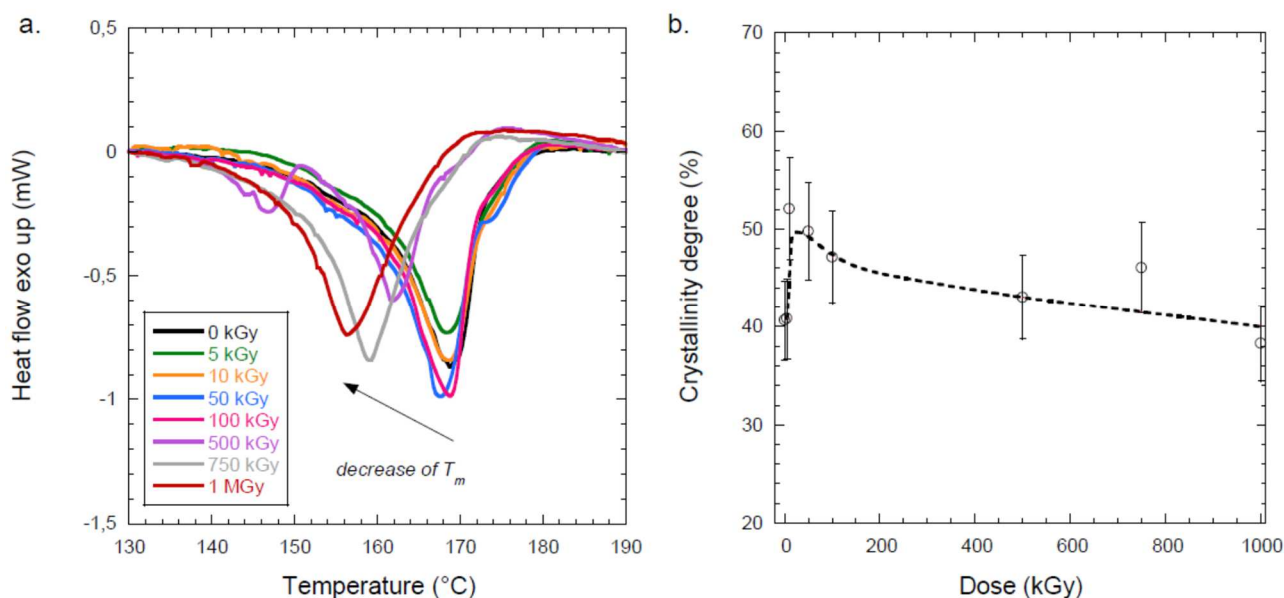
Figure 6: a. DSC melting peak for PVDF polymer films treated by different dose of irradiation, b. percentage of crystallinity in function of irradiation dose
