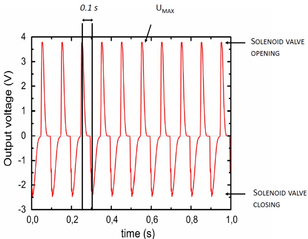
Figure 1: Example of piezopotential response during poled PVDF deformation under following conditions: f = 10\text{Hz} , R = 1\text{M}\Omega , C = 220\text{nF} , P = 0.58\text{Bar}
